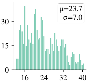
PRCP (mm/day)
