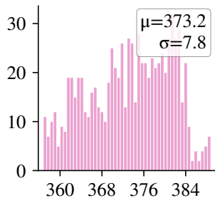
SRAD (W/m 2 )
