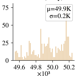
DAYL (s/day)
