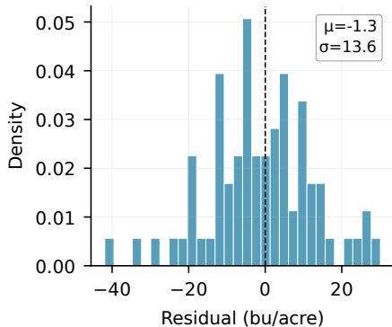
(b) Residual Distribution
