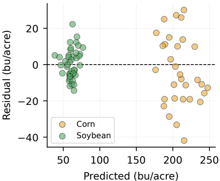
(a) Residual vs Predicted
