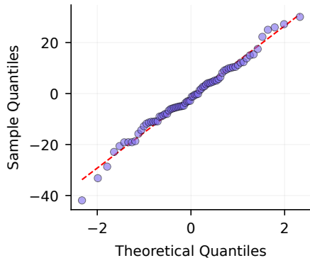
(c) Q-Q Plot
