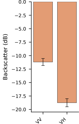
Sentinel-1
