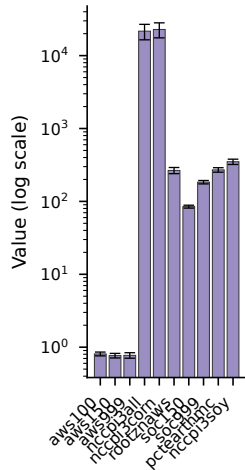
Soil
