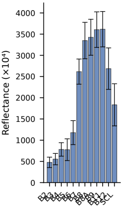
Sentinel-2
