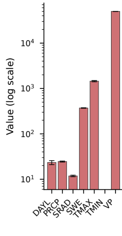
Weather
