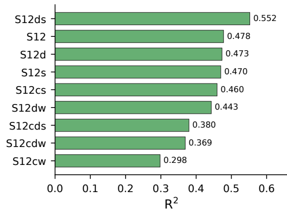
(b) Soybean — R^2 by Modality
