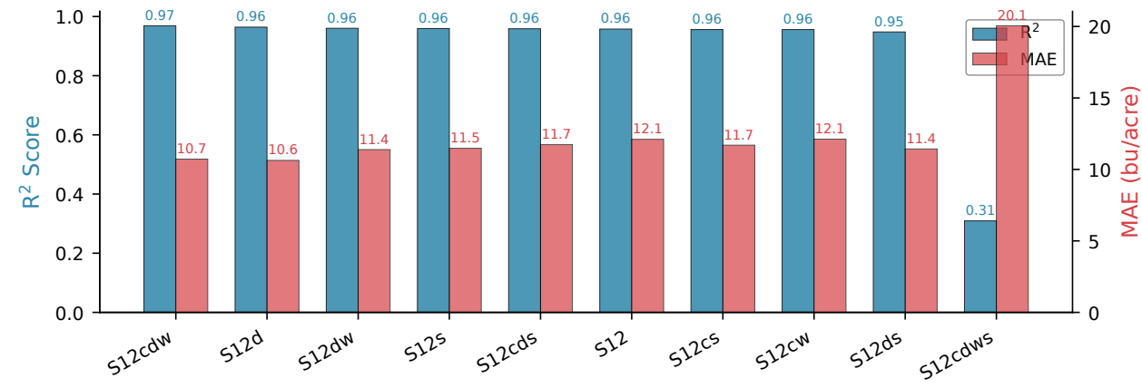
(c) Overall — R^2 and MAE by Modality Configuration
