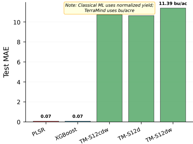
(b) MAE Comparison
