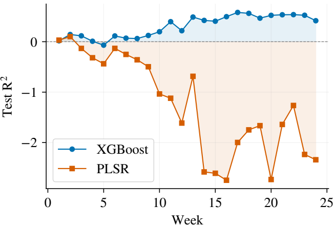
(a) Test R^2 by Week
