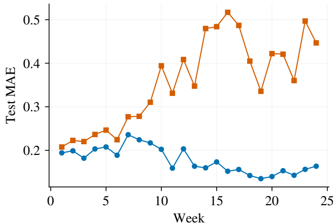
(b) Test MAE by Week
