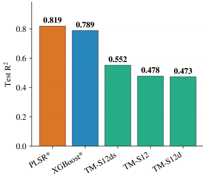
(b) Soybean — R^2 Comparison
