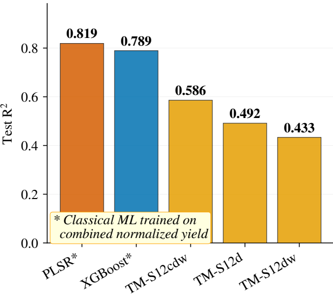
(a) Corn — R^2 Comparison
