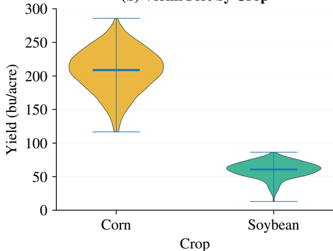
(b) Violin Plot by Crop
