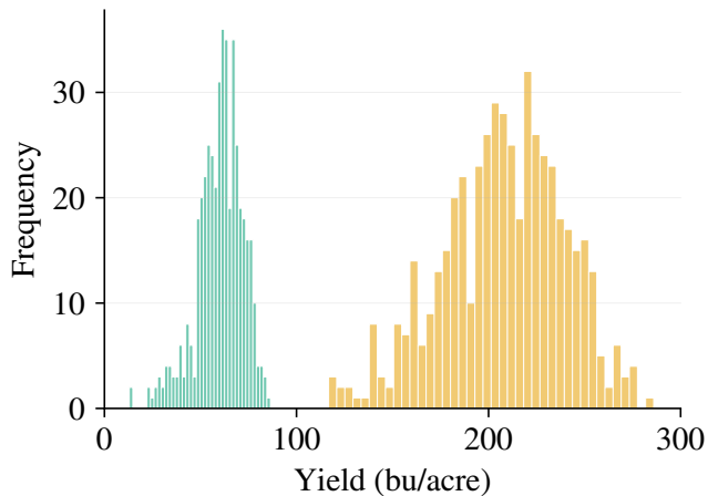
(a) Histogram — Overlapped
