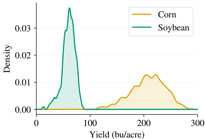
(b) KDE — Density Comparison
