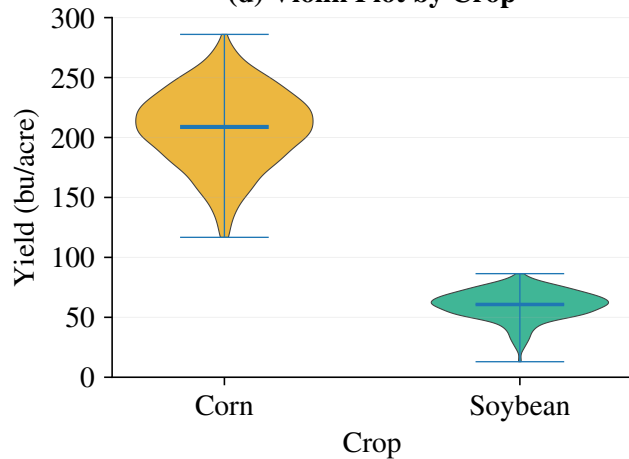
(d) Violin Plot by Crop
