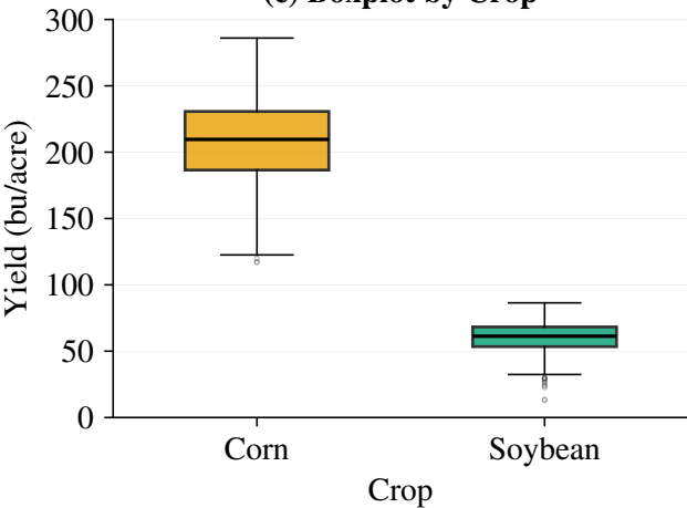
(c) Boxplot by Crop
