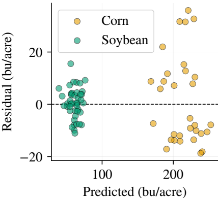
(a) Residual vs Predicted
