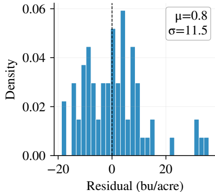
(b) Residual Distribution
