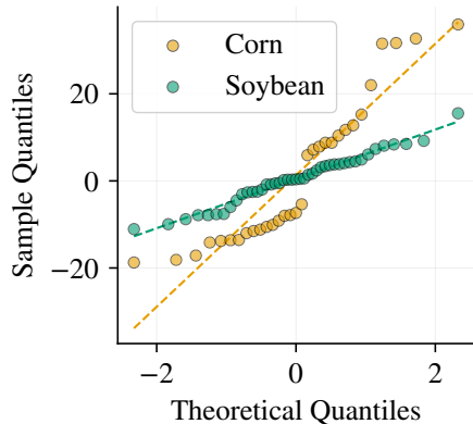
(c) Q-Q Plot (by crop)
