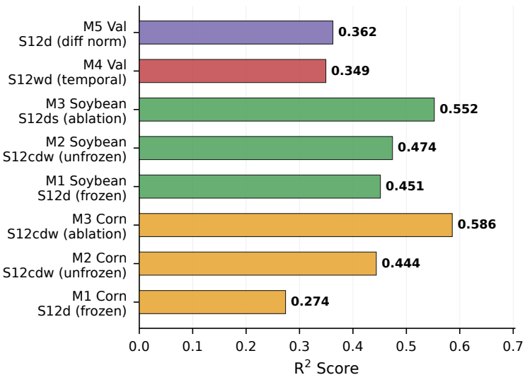
(a) R 2 Comparison
