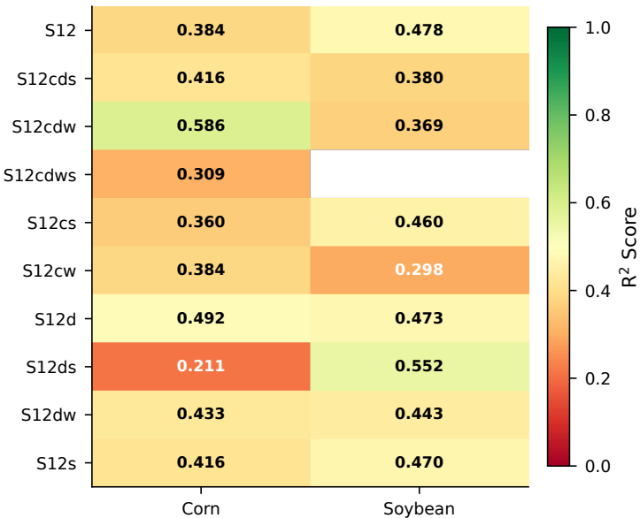
M3: Modality Ablation R 2 Heatmap
