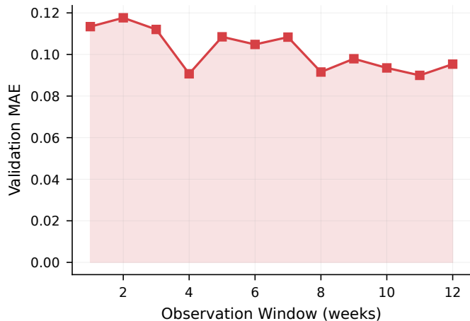
(b) MAE vs Temporal Window
