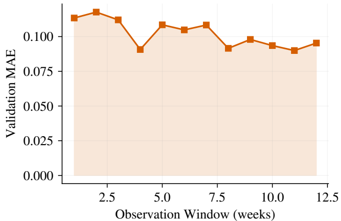
(b) MAE vs Temporal Window
