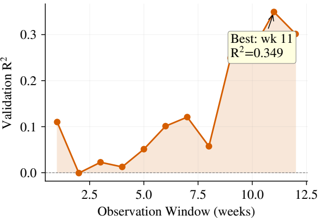
(a) R^2 vs Temporal Window
