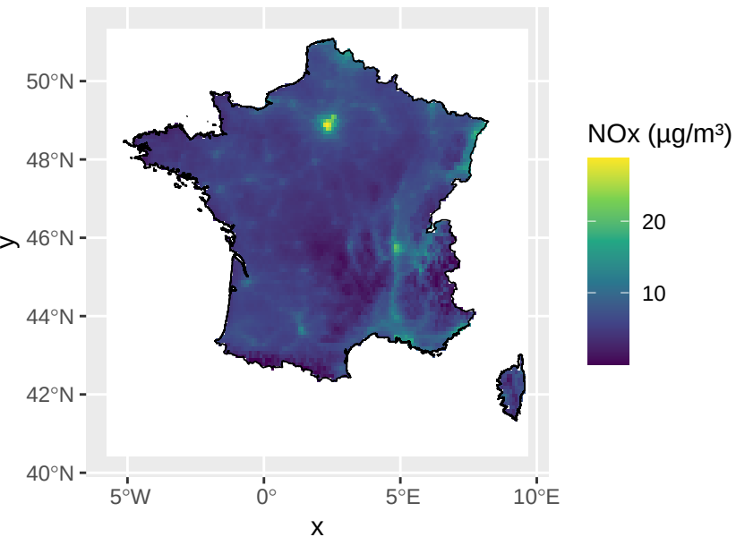
Average NO x Concentration 2022 -- France (downsampled)
