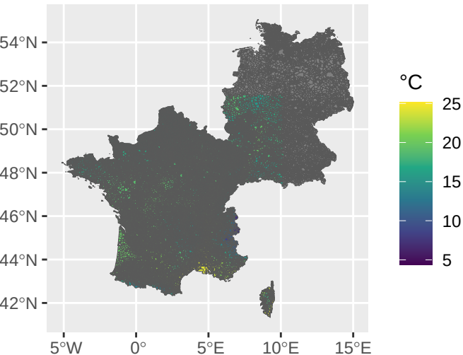
Mean July Temperature -- stars::aggregate() approach
