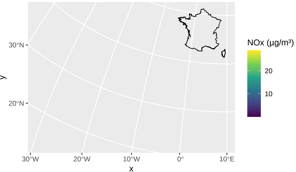
Average NOx Concentration 2022 -- France (downsampled)
