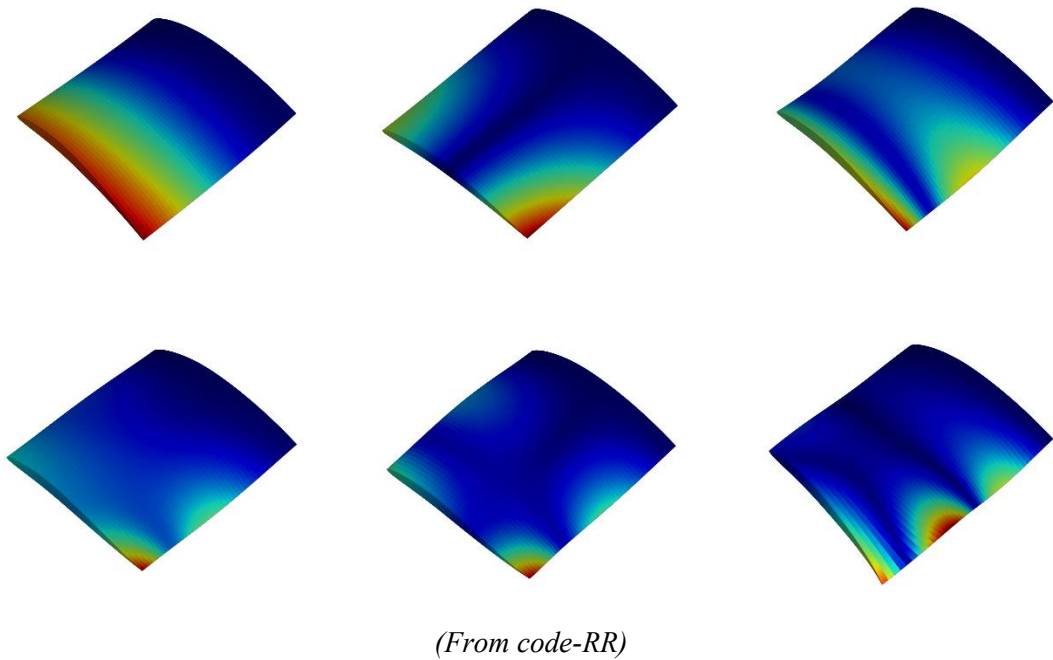
Figure 5 — Non-rotating mode shapes: present versus ANSYS. Caption: Side-by-side deformed skins for the lowest six modes, colored by displacement magnitude on a common scale. Identify each mode by its dominant character (first flap, first edgewise, first torsion, second flap, chordwise bending, coupled flap–torsion) and comment on the flap–torsion coupling induced by pre-twist and the stacking-axis offset from the section centroid. Report the Modal Assurance Criterion between corresponding present and FE mode shapes evaluated on a common grid of mid-surface points.
