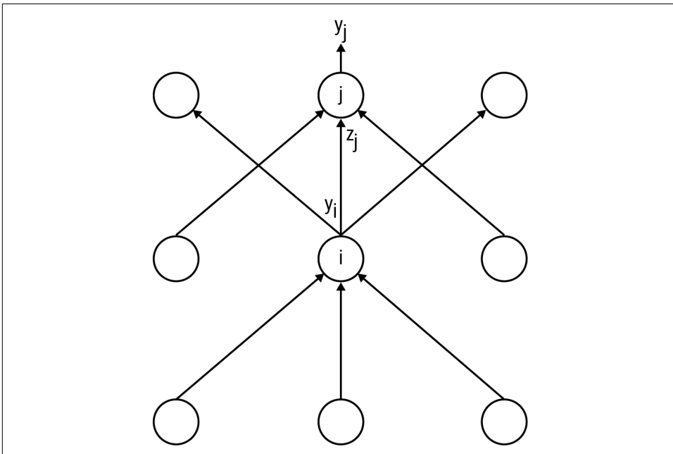
Figure 4-5. Reference diagram for the derivation of the backpropagation algorithm
