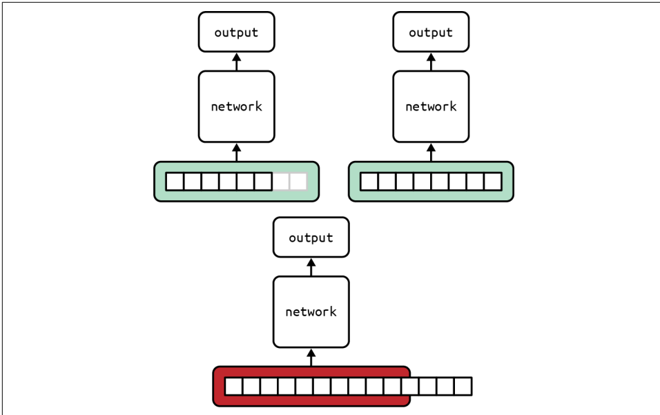
Figure 9-1. Broken feed-forward network
