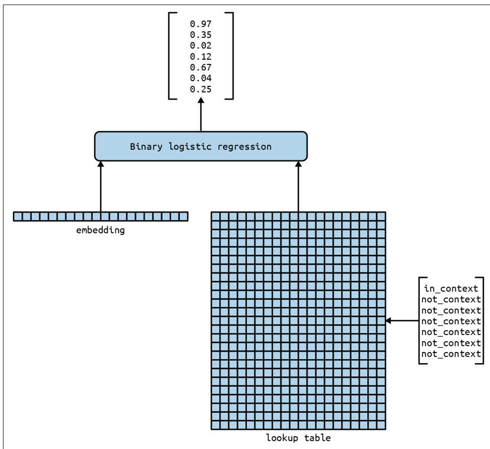
Figure 8-20. The NCE strategy
