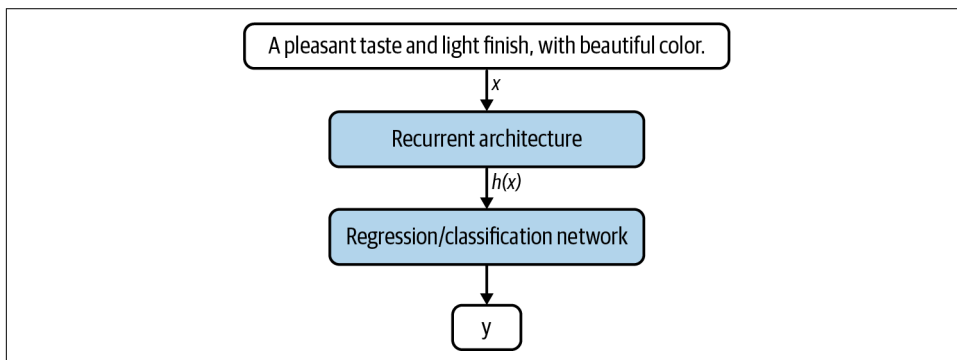
Figure 11-4. Depicted is the classical property predictor, where x is an encoding of the original sentence, h(x) is the hidden state produced by the recurrent architecture after reaching the end of x , and y is the result of a standard feed-forward neural architecture.
