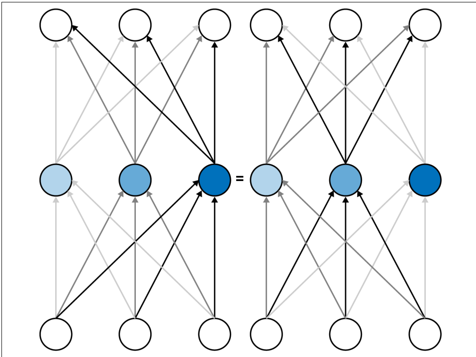
Figure 6-2. Rearranging neurons in a layer of a neural network results in equivalent configurations due to symmetry
