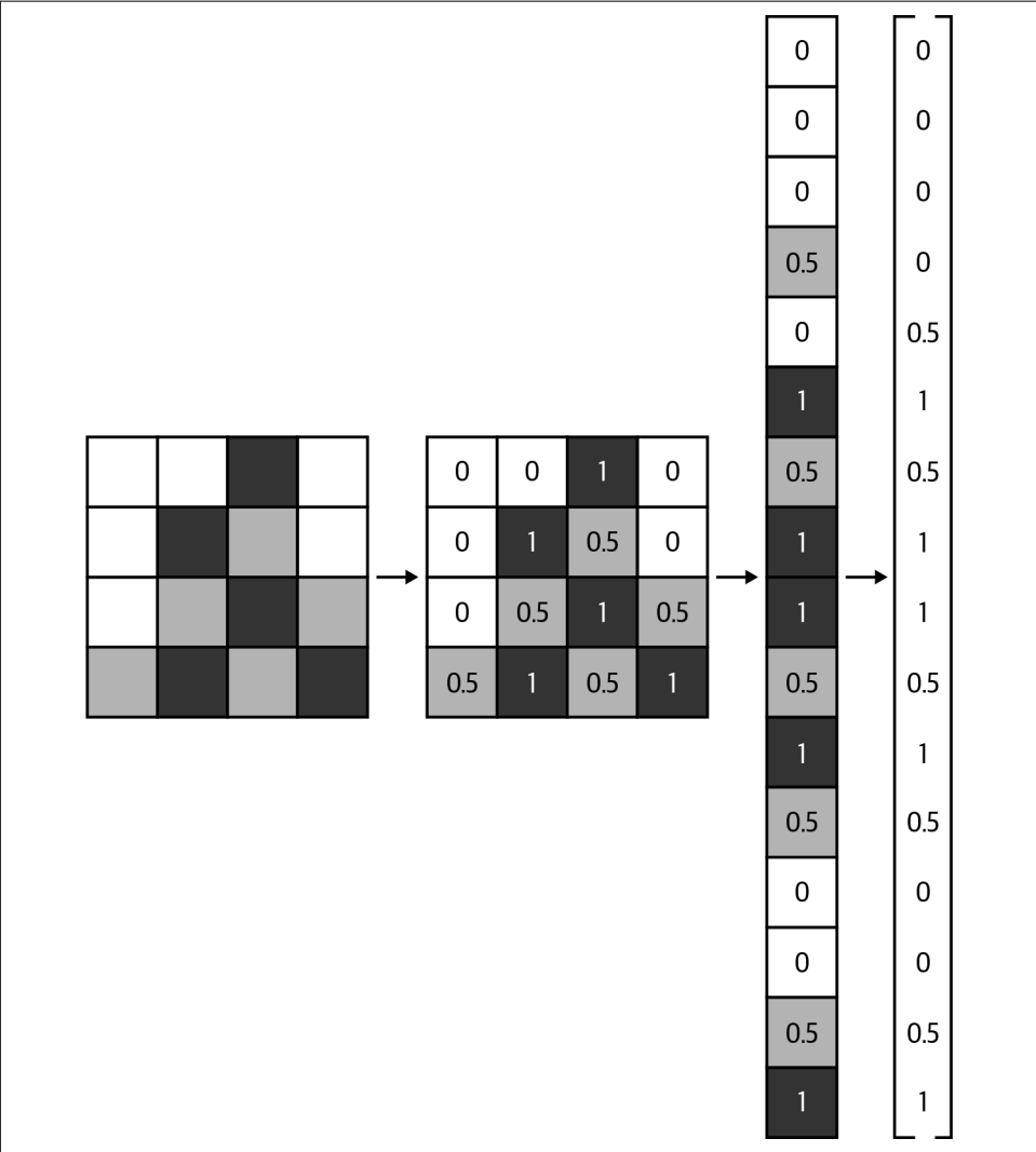
Figure 3-3. The process of vectorizing an image for a machine learning algorithm
