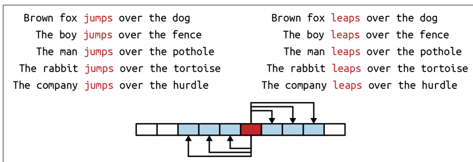
Figure 8-18. Analyzing context to determine a word's meaning
