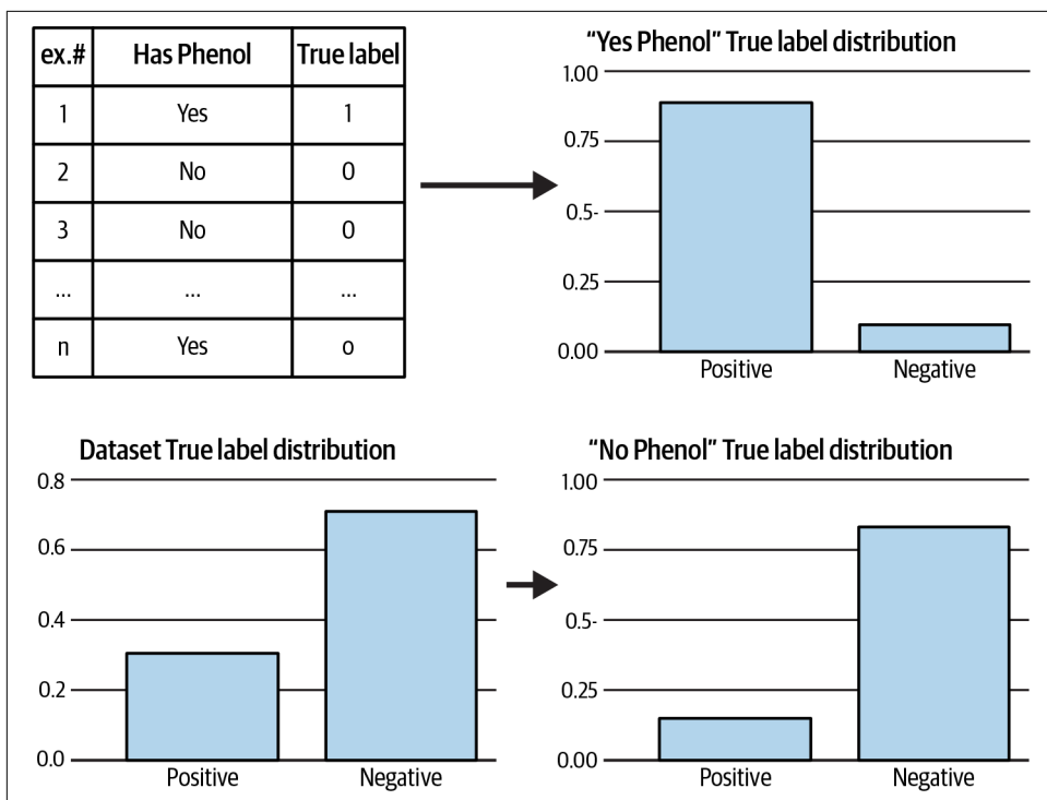
Figure 11-3. The original dataset can be broken down into 30% toxic and 70% nontoxic, where a true label of 1 indicates toxicity and 0 otherwise. Breaking up the n examples into two subgroups based on containing phenol greatly concentrates the true probability over a single label in each subgroup.
