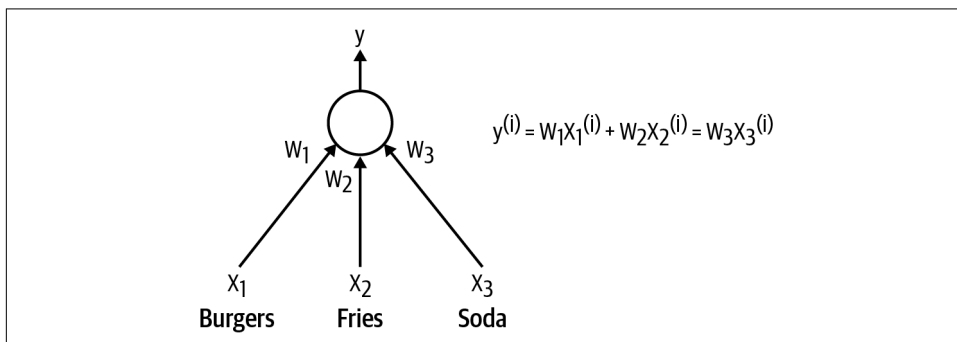
Figure 4-1. This is the neuron we want to train for the fast-food problem
