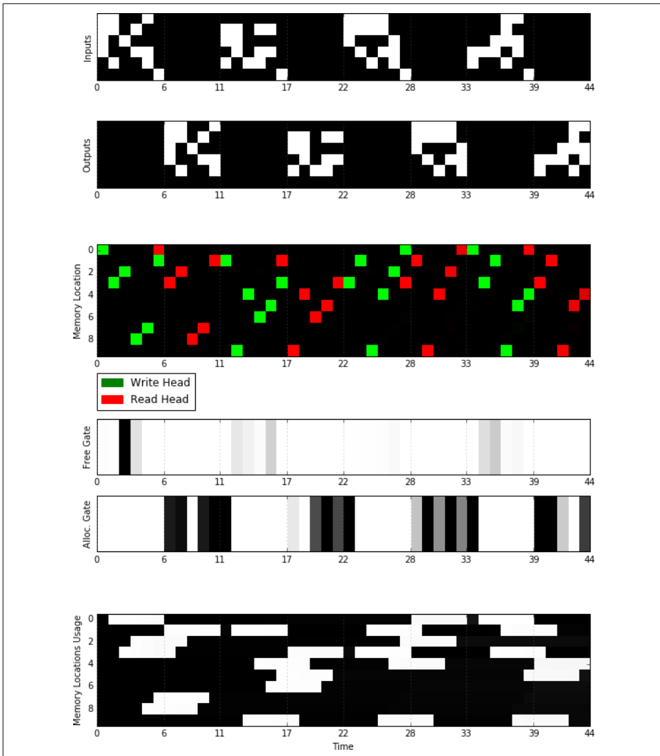
Figure 12-9. Visualization of the DNC operation on the copy problem
