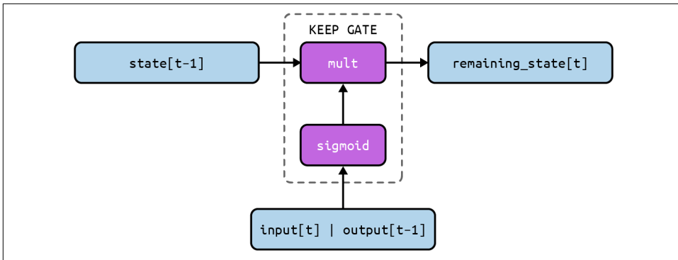
Figure 9-18. Architecture of the keep gate of an LSTM unit
