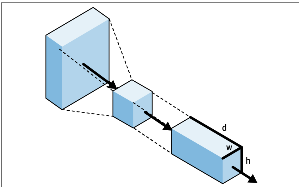
Figure 7-4. Convolutional layers arrange neurons in three dimensions, so layers have width, height, and depth
