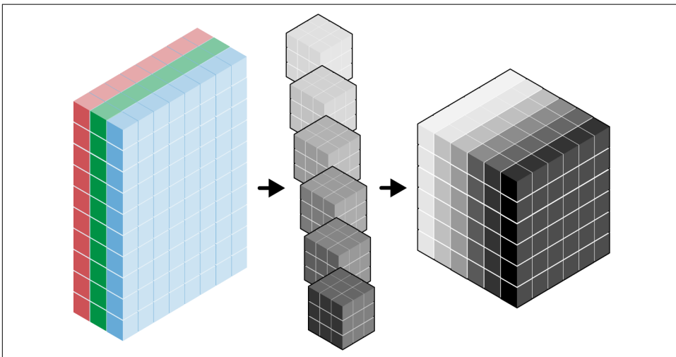
Figure 7-9. A three-dimensional visualization of a convolutional layer, where each filter corresponds to a slice in the resulting output volume
