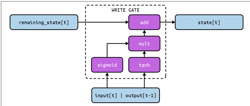
Figure 9-19. Architecture of the write gate of an LSTM unit
