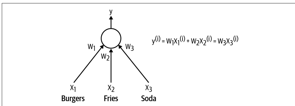
Figure 3-10. An example of a linear neuron
