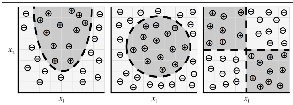
Figure 3-5. As our data takes on more complex forms, we need more complex models to describe them
