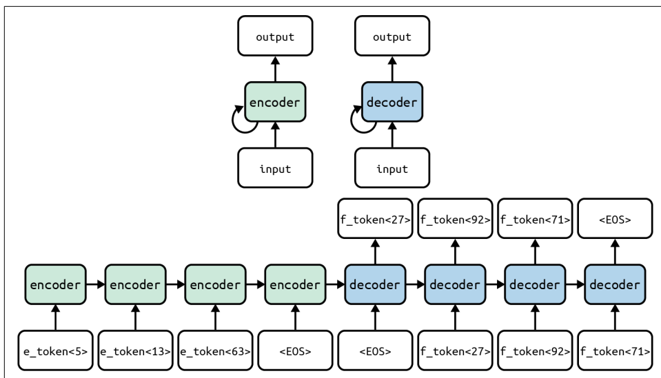
Figure 9-24. How we use an encoder/decoder recurrent network schema to tackle seq2seq problems
