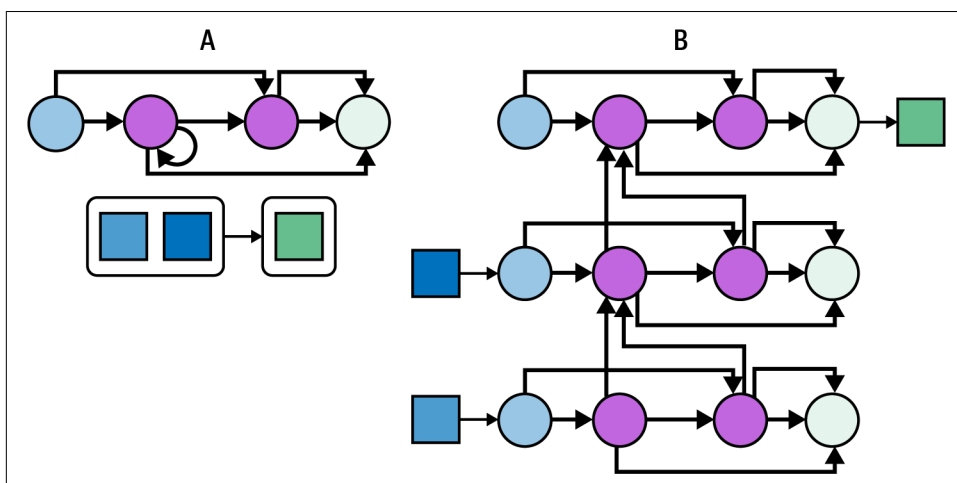
Figure 9-15. We can run an RNN through time to express it as a feed-forward network that we can train using backpropagation
