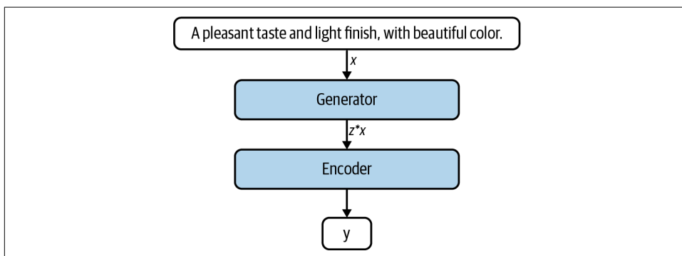
Figure 11-5. The generator parametrizes a distribution over masks z given input x , which we sample from to get the input to the encoder. The encoder follows the same structure as that of the classical property predictor depicted earlier.
