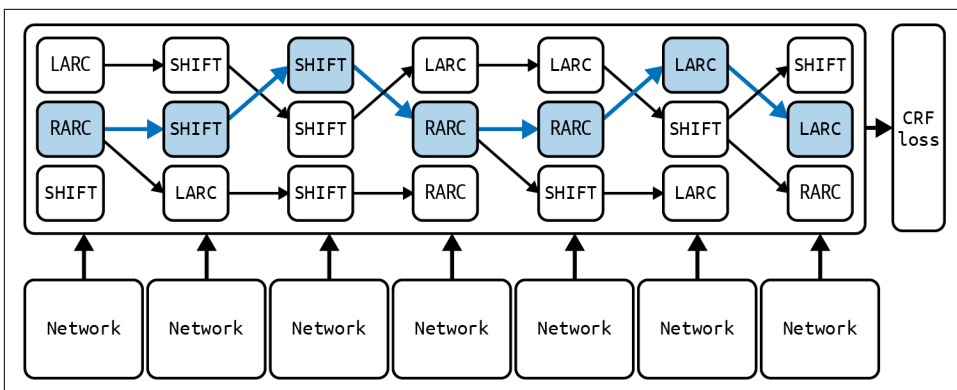
Figure 9-12. Coupling training and beam search can make global normalization in SyntaxNet tractable
