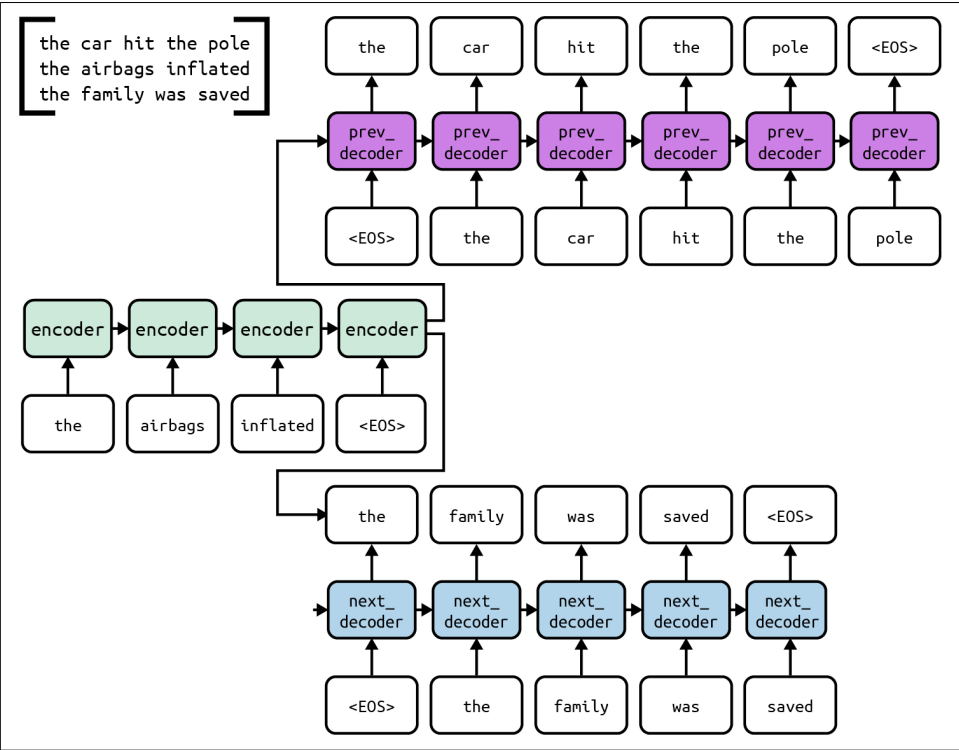
Figure 9-25. The skip-thought seq2seq architecture to generate embedding representations of entire sentences
