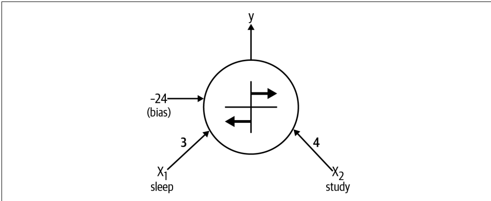
Figure 3-8. Expressing our exam performance perceptron as a neuron
