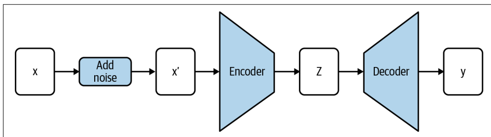
Figure 10-8. The denoising autoencoder architecture is the same as that of the standard autoencoder, except instead of minimizing the reconstruction error between y and the input x' , we minimize the reconstruction error between y and the original x .
