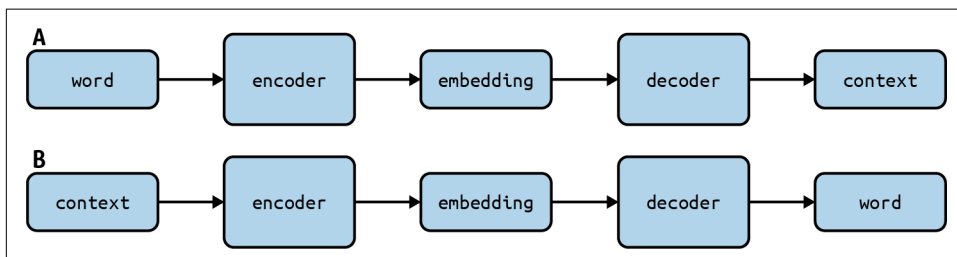
Figure 8-19. General architectures for designing encoders and decoders that generate embeddings by mapping words to their respective contexts (A) or vice versa (B)
