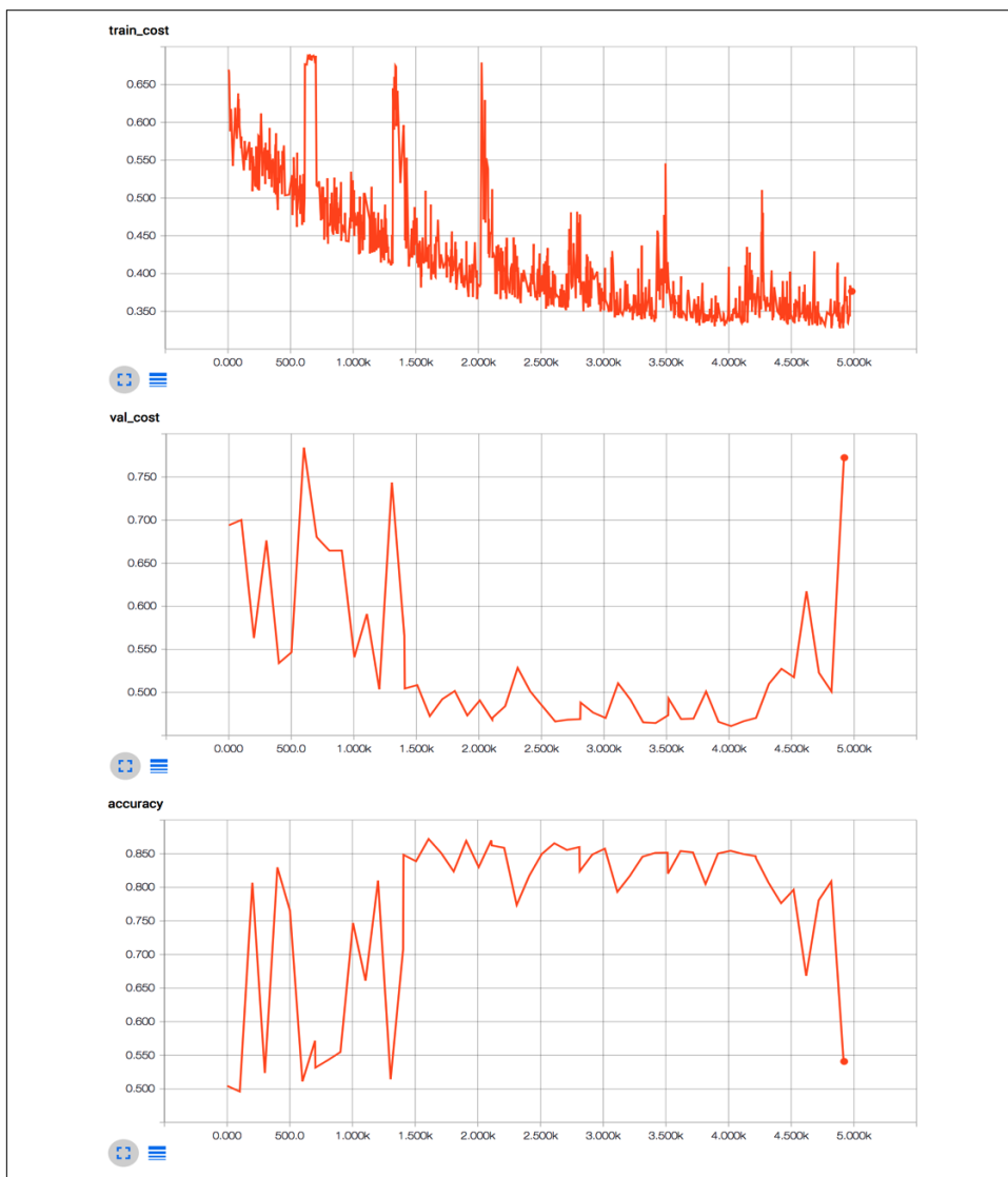
Figure 9-23. Training cost, validation cost, and accuracy of our movie review sentiment model
