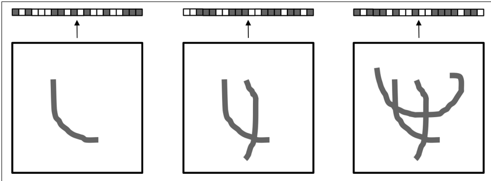
Figure 8-15. The activations of a dense representation combine and overlay information from multiple features in ways that are difficult to interpret
