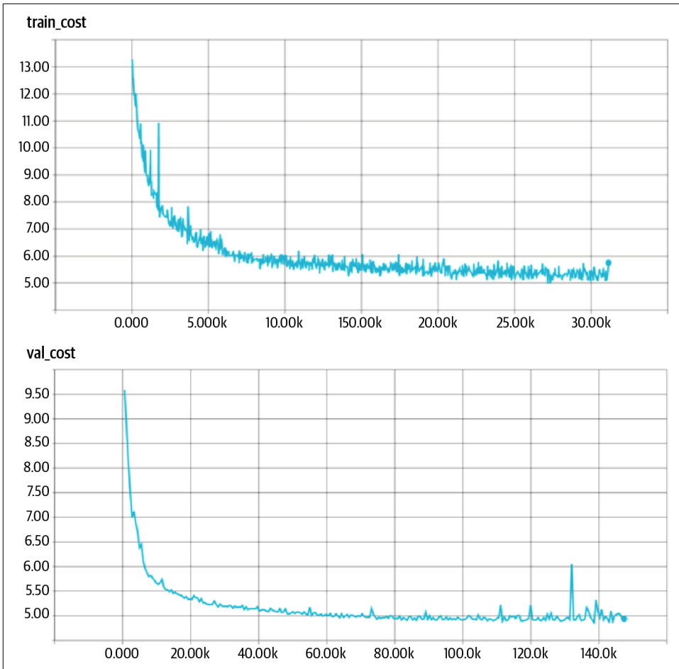
Figure 8-7. The cost incurred on the training set (logged after each minibatch) and on the validation set (logged after each epoch)
