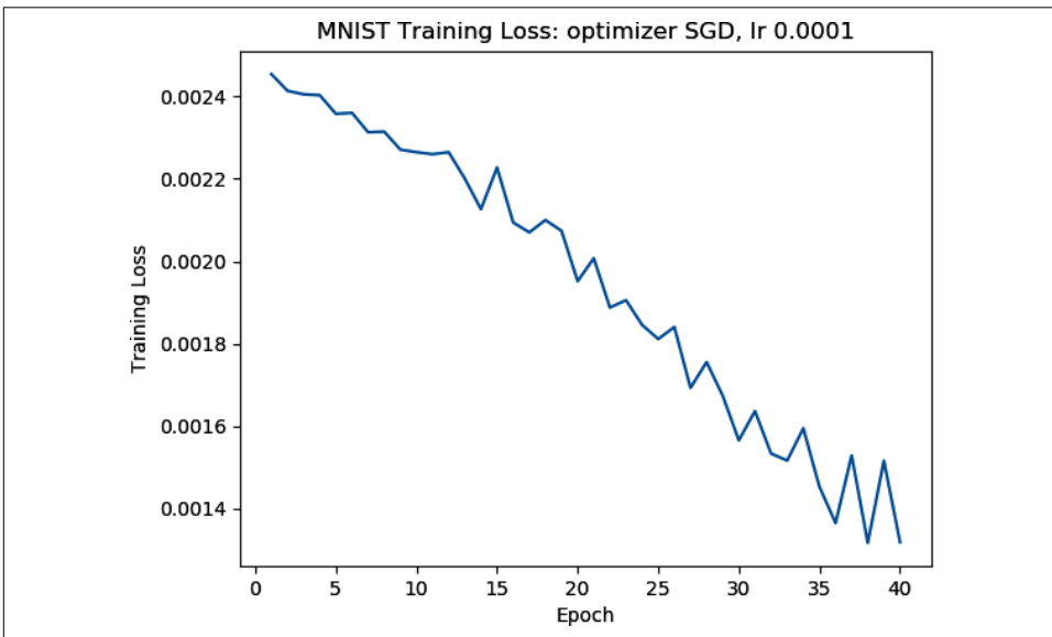
Figure 5-2. We see signs of underfitting as the model performance on the training set is failing to level out, meaning we have not yet settled into a local optimum
