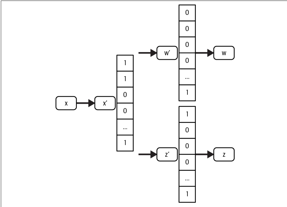
Figure 11-6. x can be thought of as some high-dimensional input such as an image, while each index of x' is associated with some interpretable feature, where a 1 denotes the existence of that feature in x . The sampling procedure selects some subset of nonzero indices in x' to keep nonzero in each of w' and z' , which are then mapped back to the original input space.
