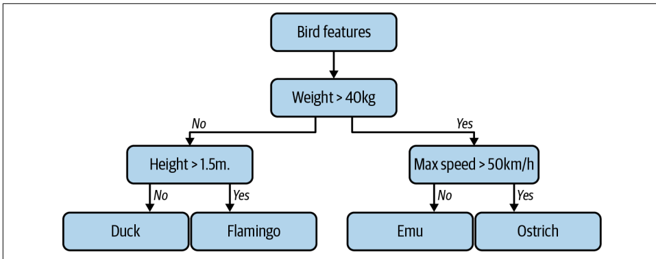
Figure 11-1. A decision tree trained to classify bird species. Given a set of bird features, follow the right “Yes” or “No” branch at each node to reach a final classification.
