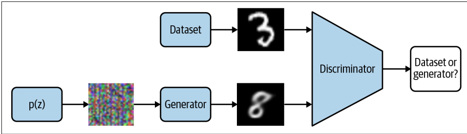
Figure 10-1. The discriminator determines whether any input image was sampled from the dataset or generator. The generator’s goal is to trick the discriminator into believing its images were sampled from the dataset.
