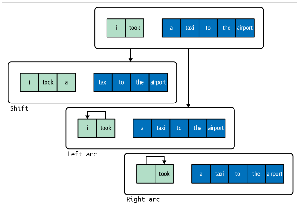
Figure 9-8. Three options in the arc-standard system: shift a word from the buffer to the stack, draw an arc from the right element to the left element (left arc), or draw an arc from the left element to the right element (right arc)
