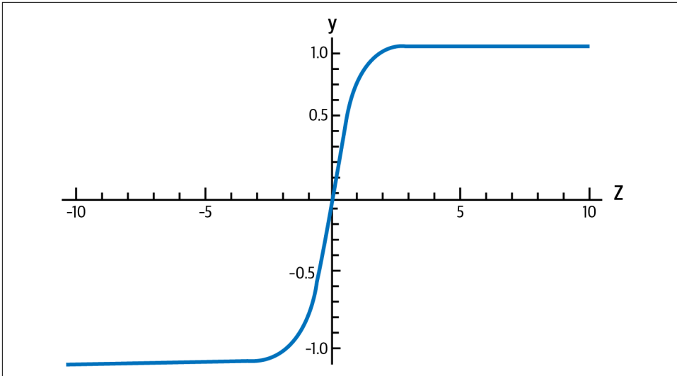
Figure 3-12. The output of a tanh neuron as z varies
