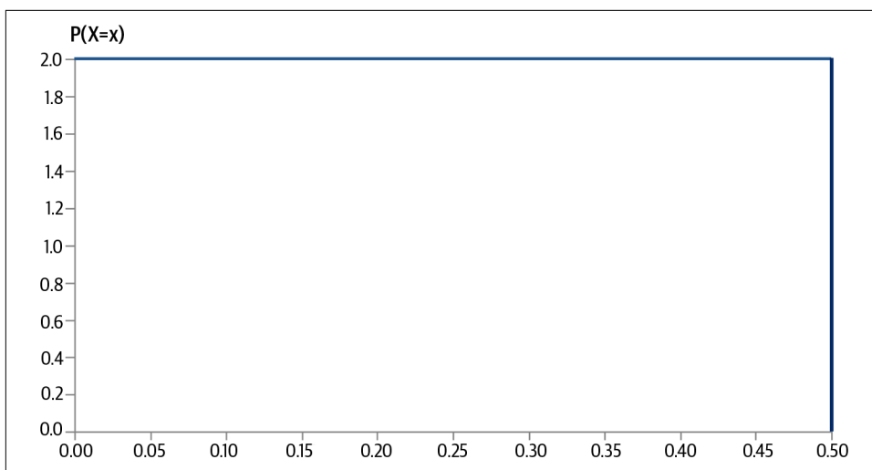
Figure 2-4. The uniform distribution has uniform height over its entire area, which shows that each value in the domain of the distribution has equal likelihood.
