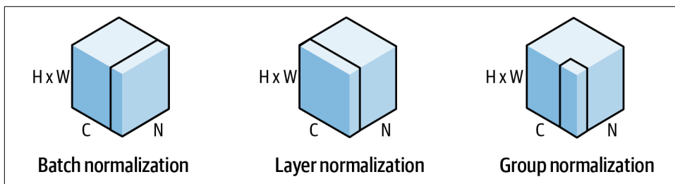
Figure 7-16. Comparison of batch normalization, layer normalization, and group normalization
