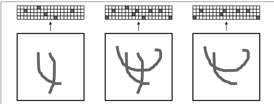
Figure 8-16. How activations in the representation change with the addition and removal of strokes
