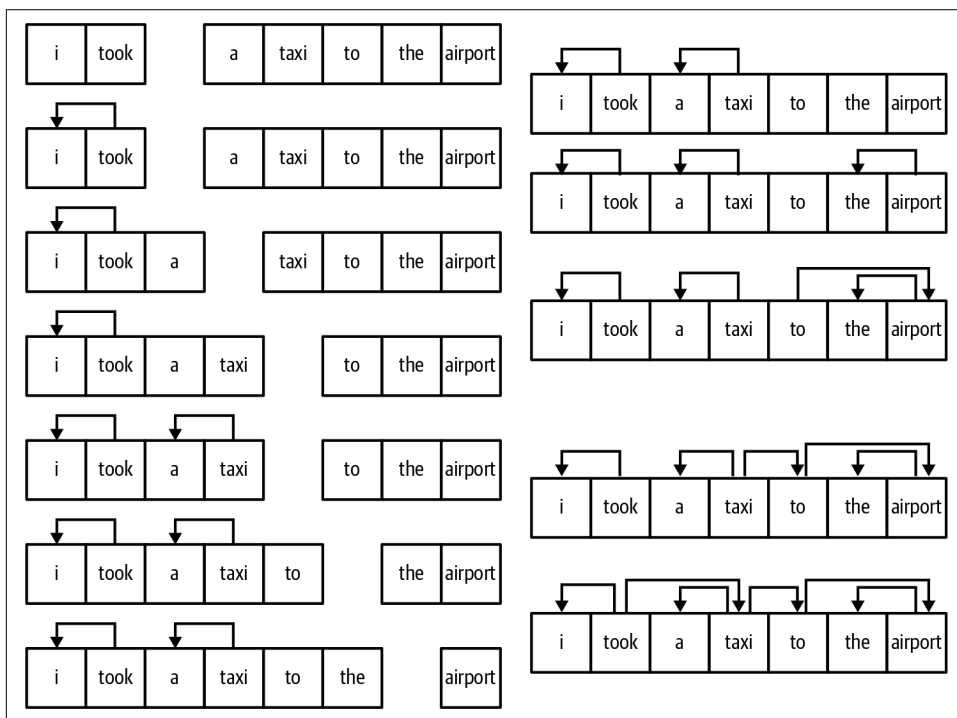
Figure 9-9. A sequence of actions that results in the correct dependency parse; we omit labels
