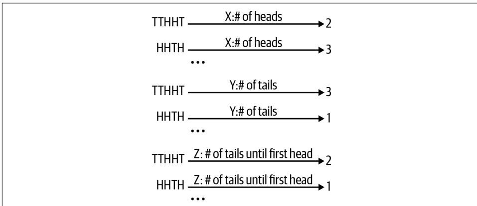
Figure 2-3. Random variables X , Y , and Z all act on the same sample space, but have varying outputs. It's important to keep in mind what you're measuring!
