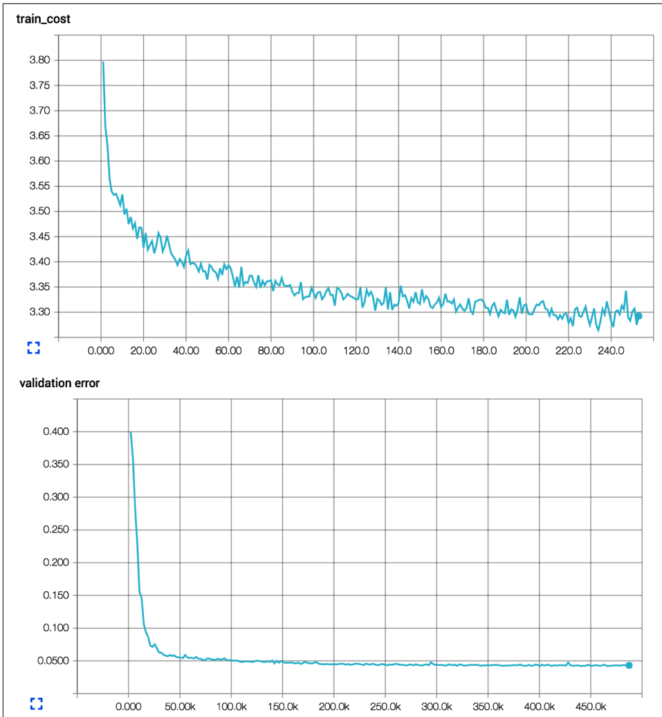
Figure 9-4. TensorBoard visualization of our feed-forward POS tagging model
