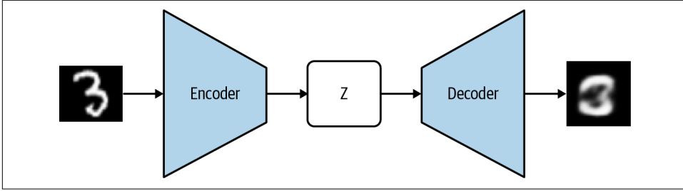
Figure 10-4. The overall VAE architecture presented in Kingma and Welling. Note that both z and the image after the decoder are both samples from the encoder distribution and decoder distribution, respectively.
