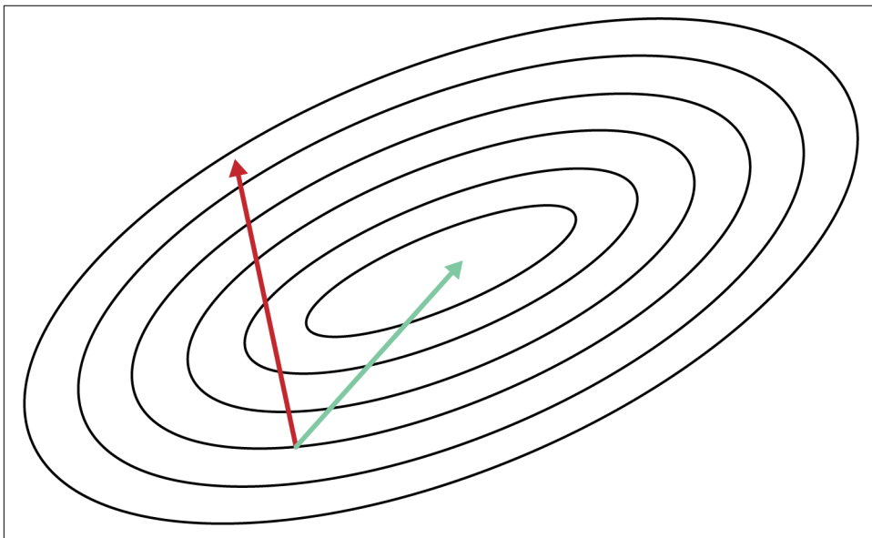
Figure 6-6. Local information encoded by the gradient usually does not corroborate the global structure of the error surface
