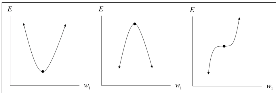
Figure 6-4. Analyzing a critical point along a single dimension
