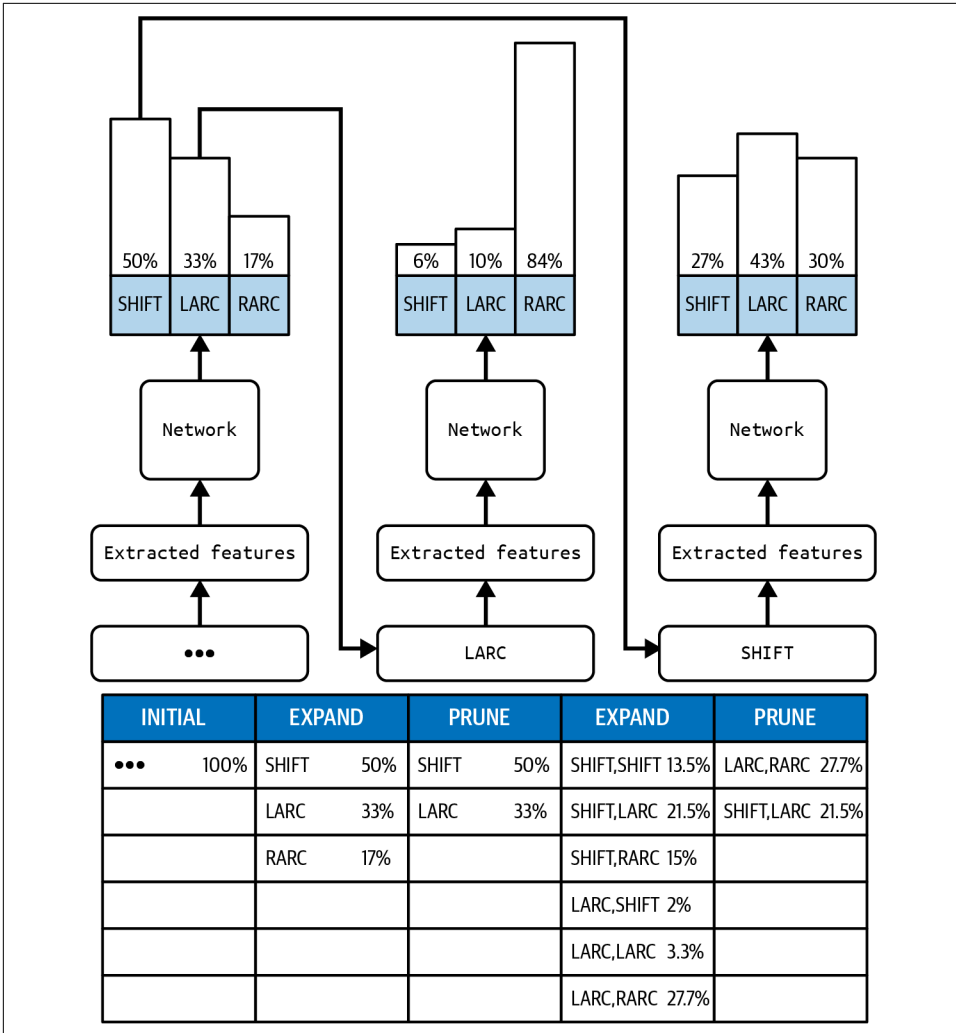
Figure 9-11. Using beam search (with beam size 2) while deploying a trained SyntaxNet model
