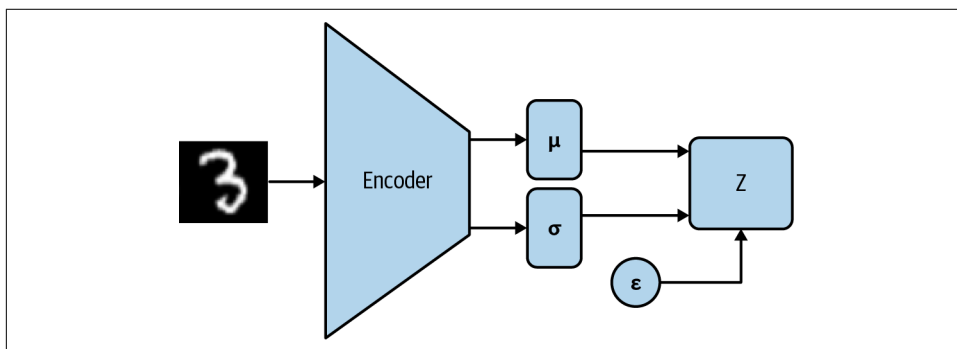
Figure 10-5. What the encoder looks like after the inclusion of reparametrization. It returns a mean and standard deviation vector, which we can combine with \epsilon to generate the setting of z . The purpose of the circle versus rectangles is to show that the only sampling is happening for \epsilon , completely independent of the encoder architecture. The mean and standard deviation vectors are produced deterministically from the input image. In addition, z is deterministic once we know the value of \epsilon .
