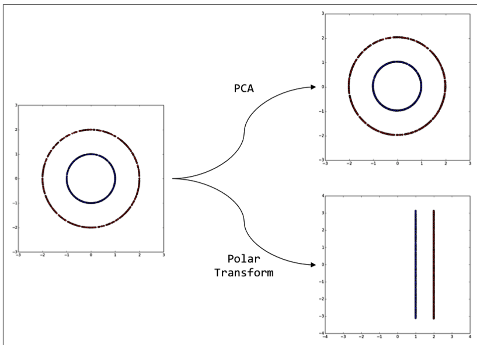
Figure 8-3. A situation in which PCA fails to optimally transform the data for dimensionality reduction
