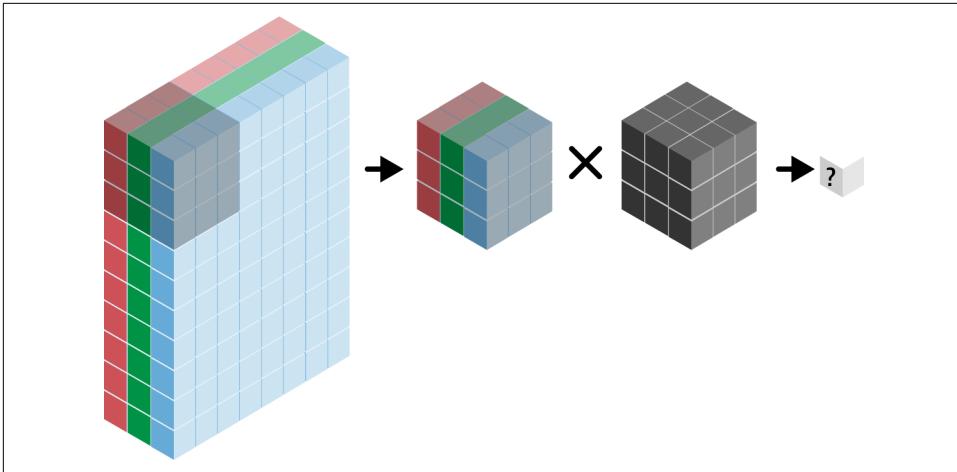
Figure 7-8. A full-color RGB image as a volume and applying a volumetric convolutional filter
