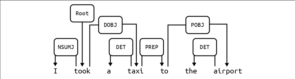
Figure 9-5. An example of a dependency parse, which generates a tree of relationships between words in a sentence
