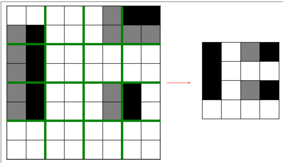
Figure 7-13. Max pooling significantly reduces parameters as we move up the network
