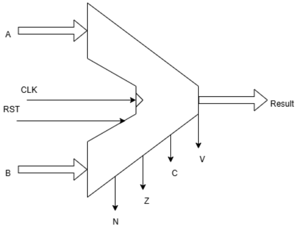
Figure 1: ALU BLock Diagram
