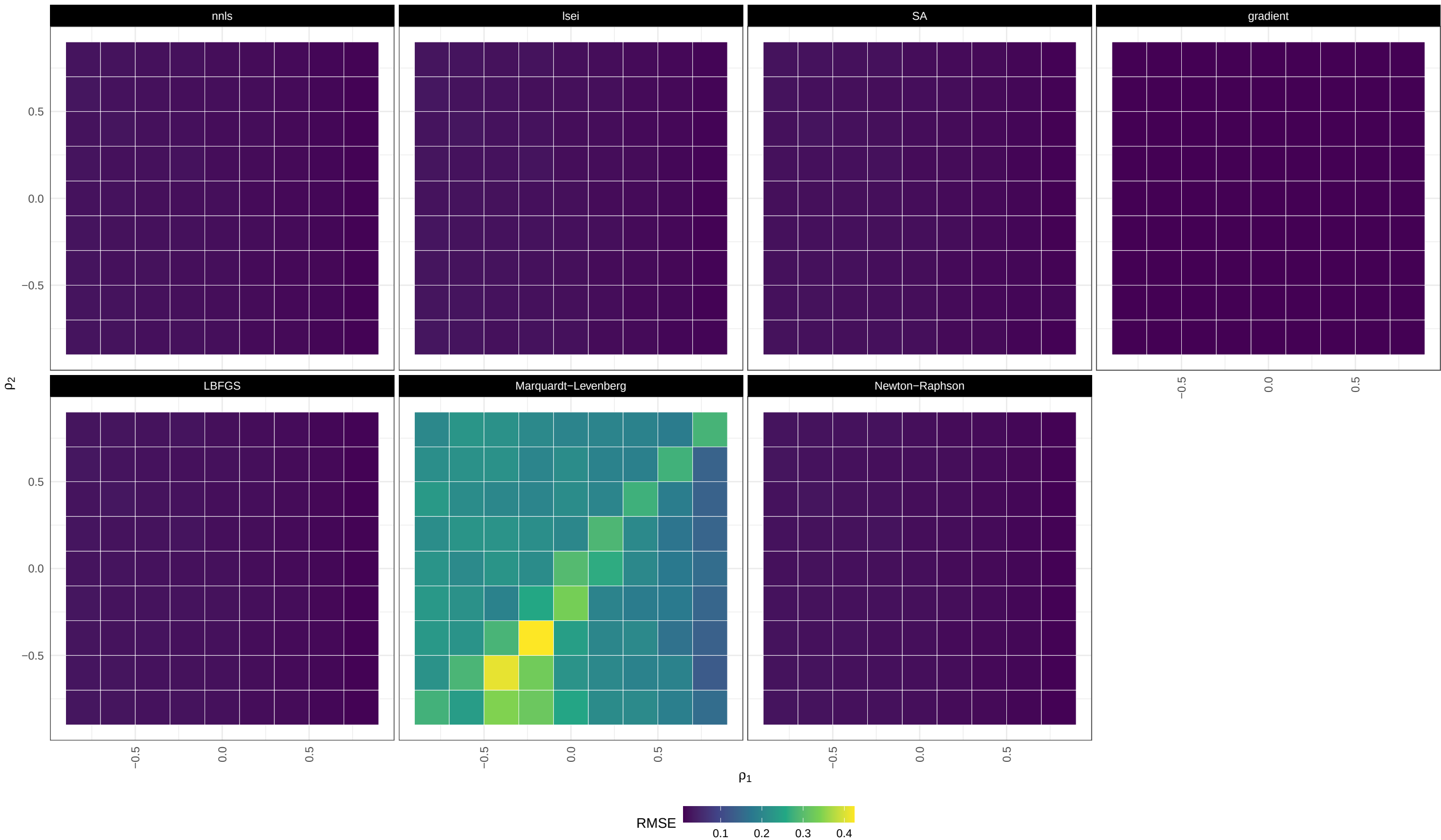
RMSE / large_CLD / heteroscedastic / highly unbalanced
