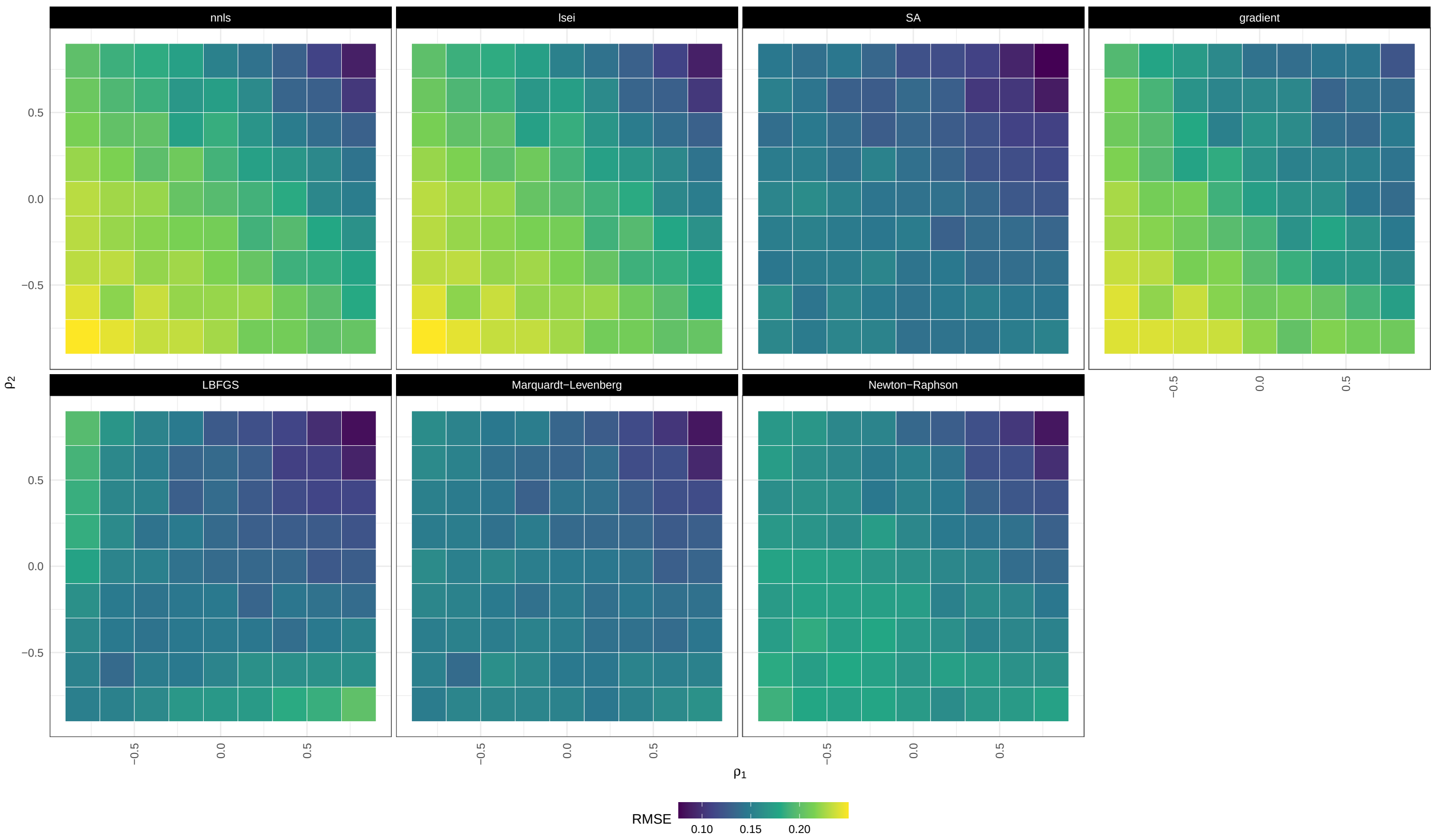
RMSE / small_CLD / homoscedastic / balanced
