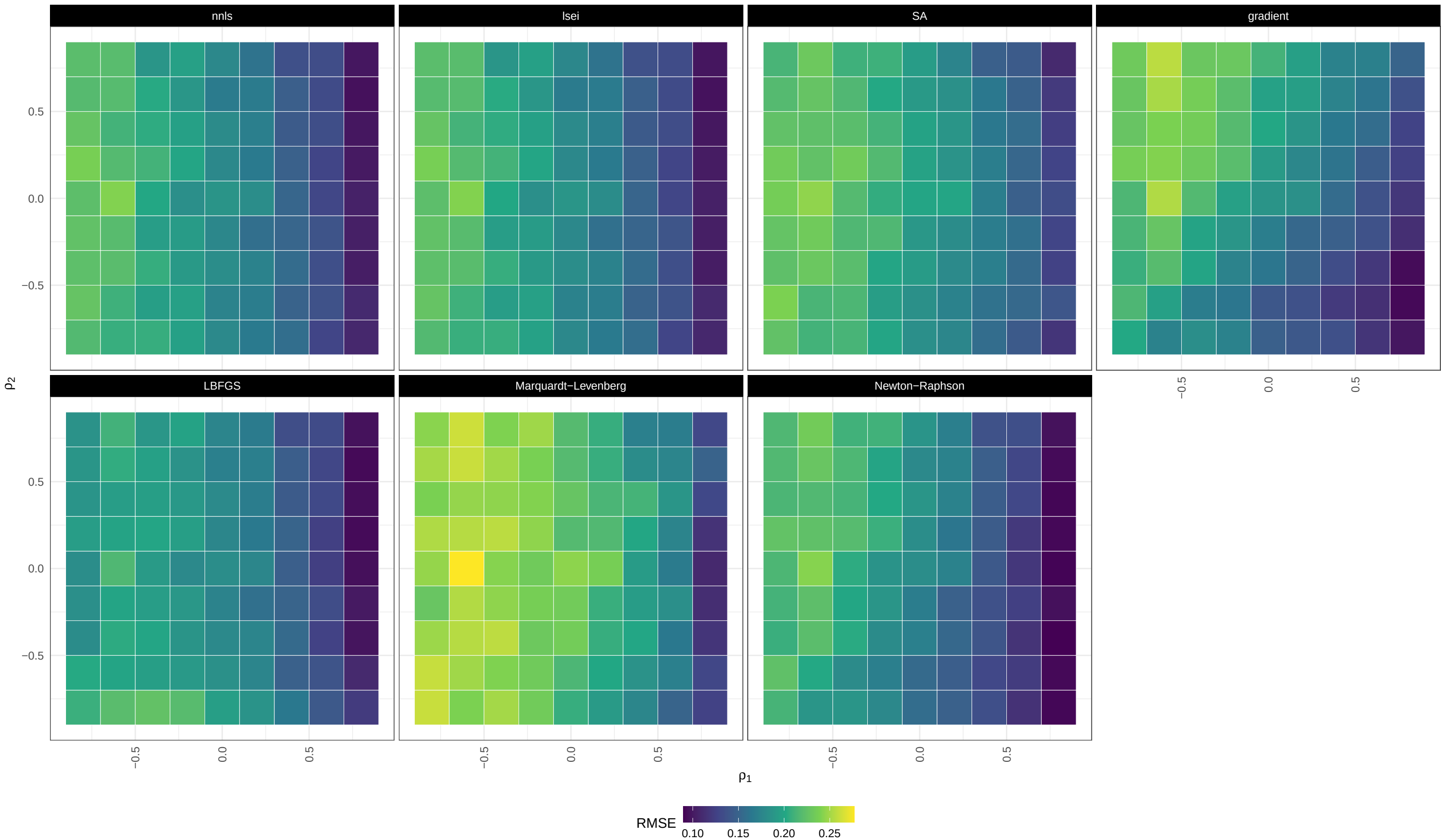
RMSE / small_CLD / homoscedastic / moderately unbalanced
