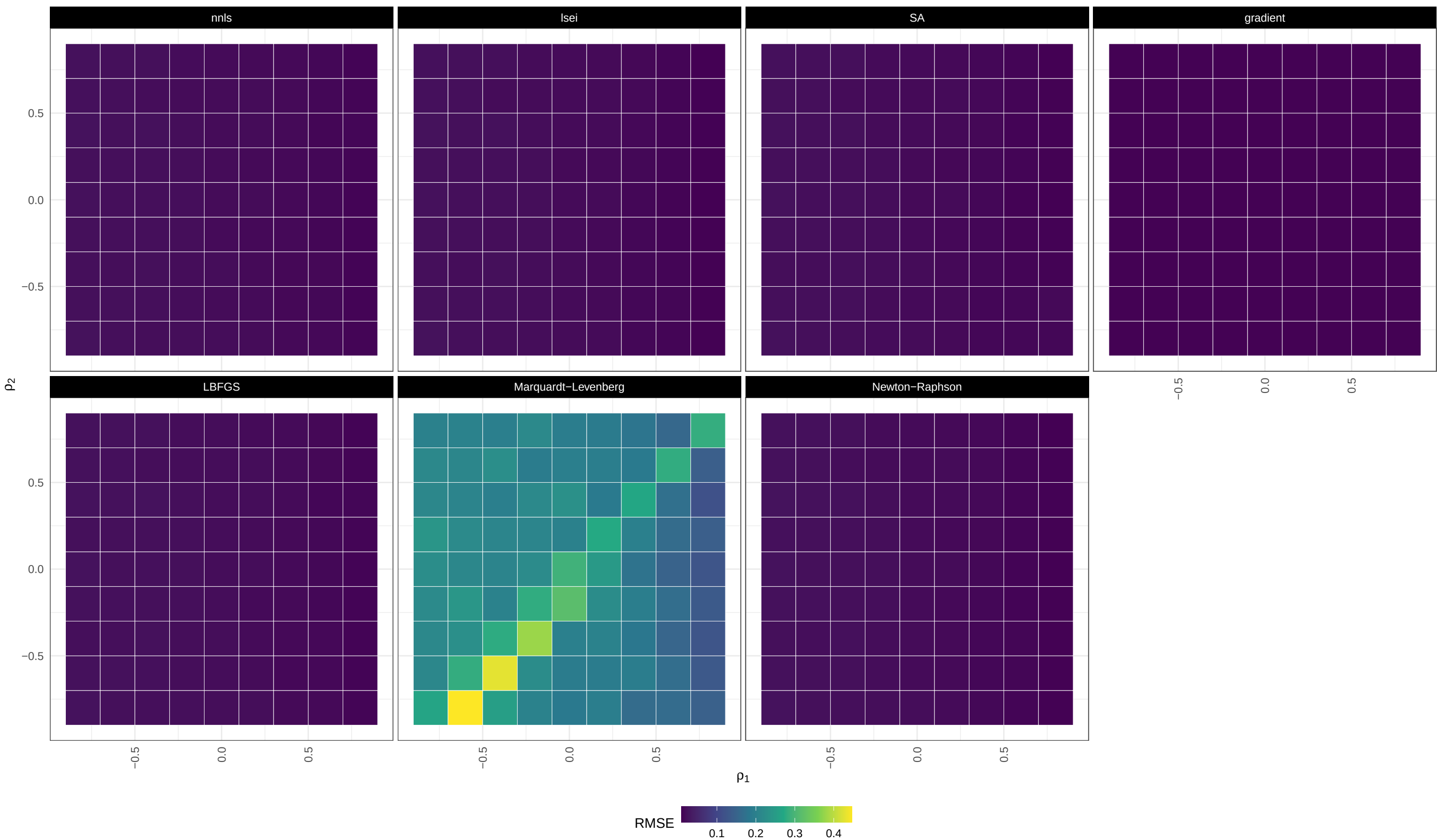
RMSE / large_CLD / homoscedastic / highly unbalanced
