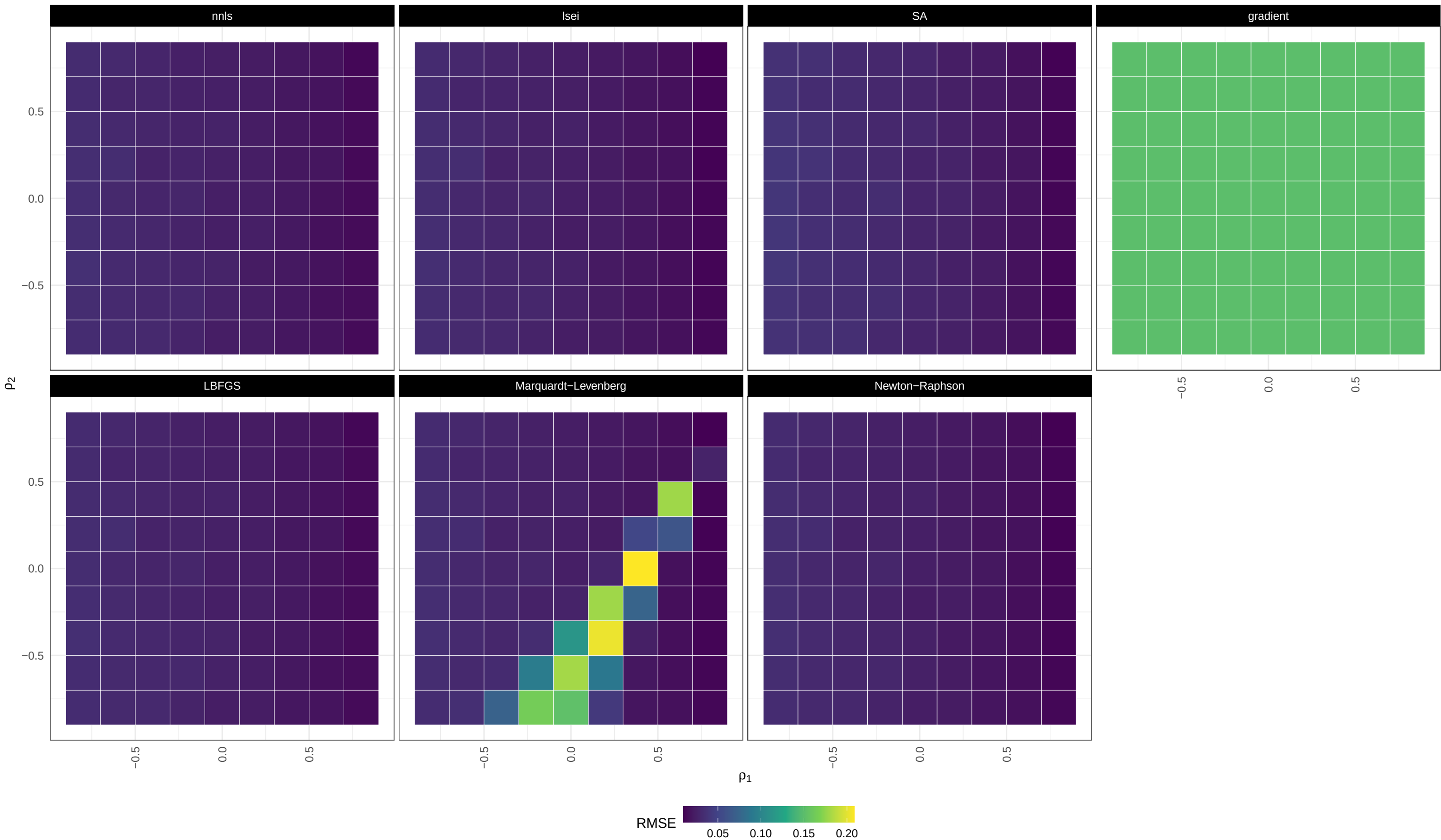
RMSE / large_CLD / homoscedastic / moderately unbalanced
