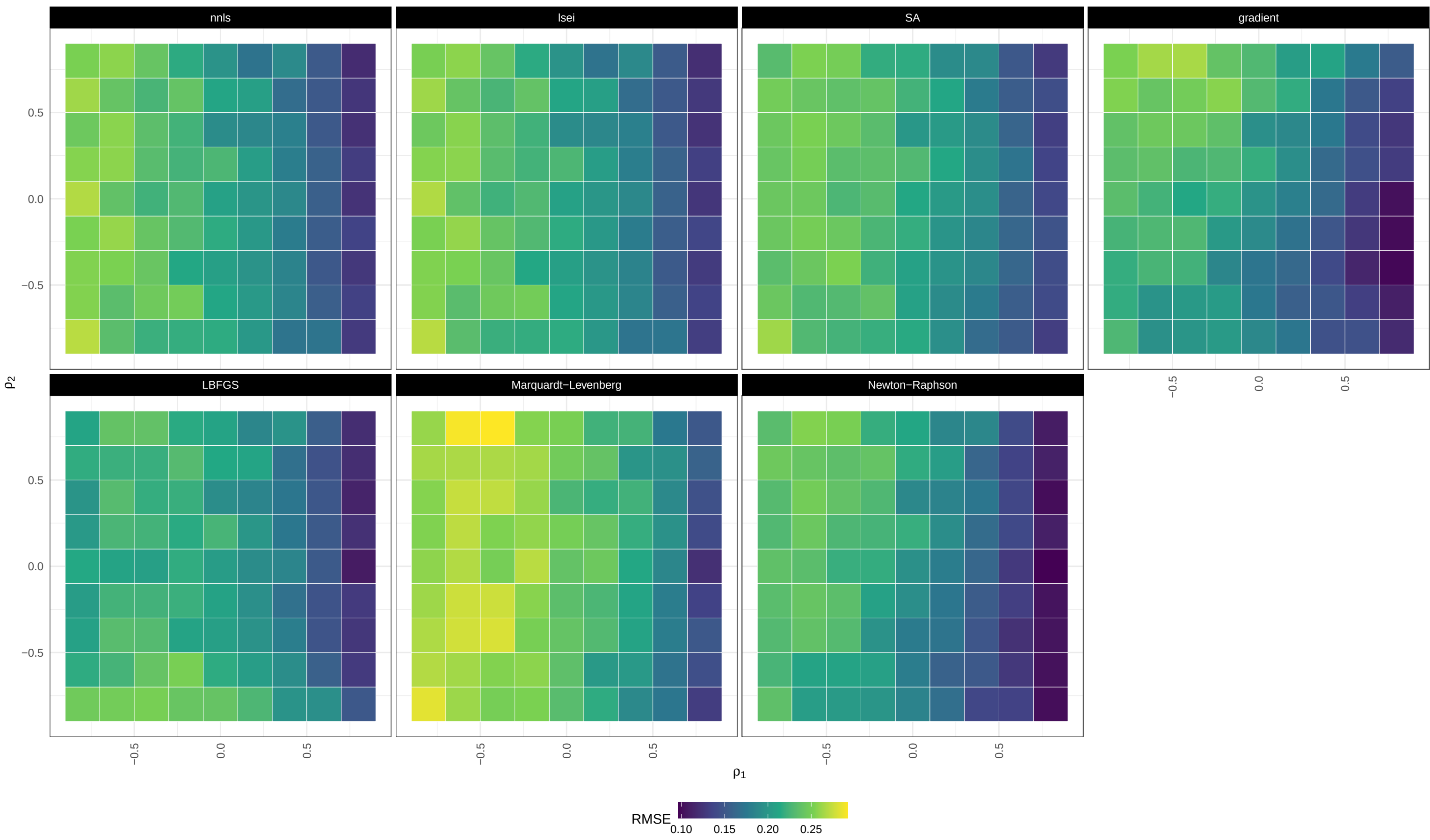
RMSE / small_CLD / heteroscedastic / moderately unbalanced
