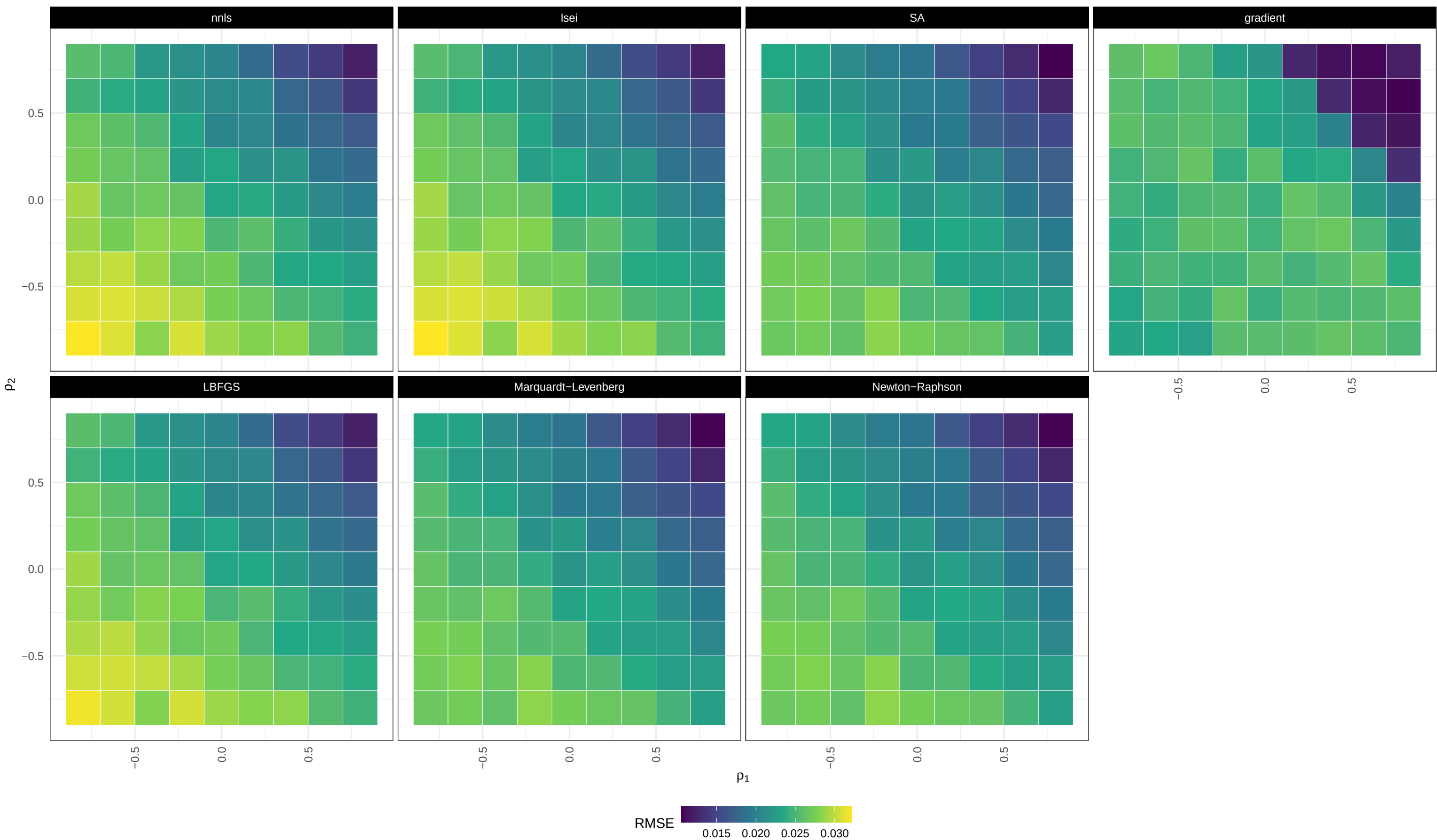
RMSE / large_CLD / heteroscedastic / balanced
