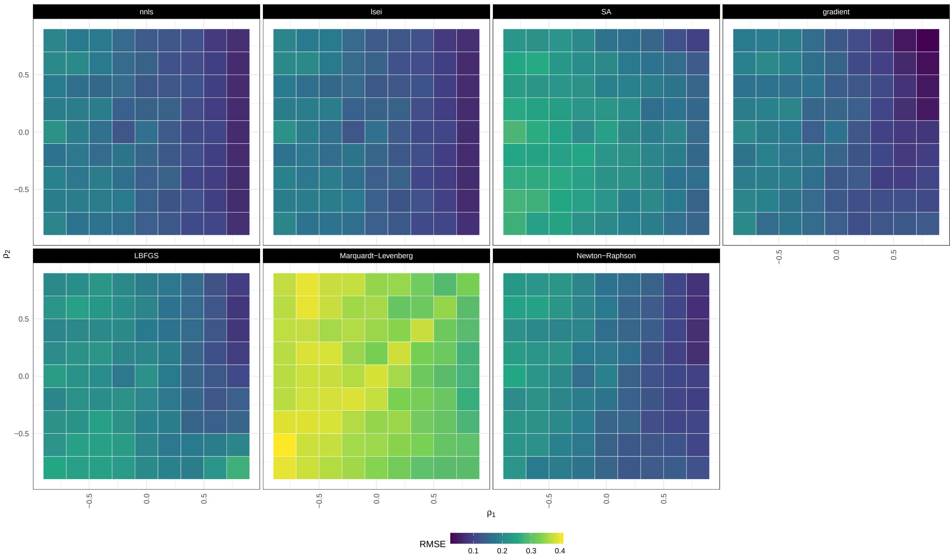
RMSE / small_CLD / homoscedastic / highly unbalanced
