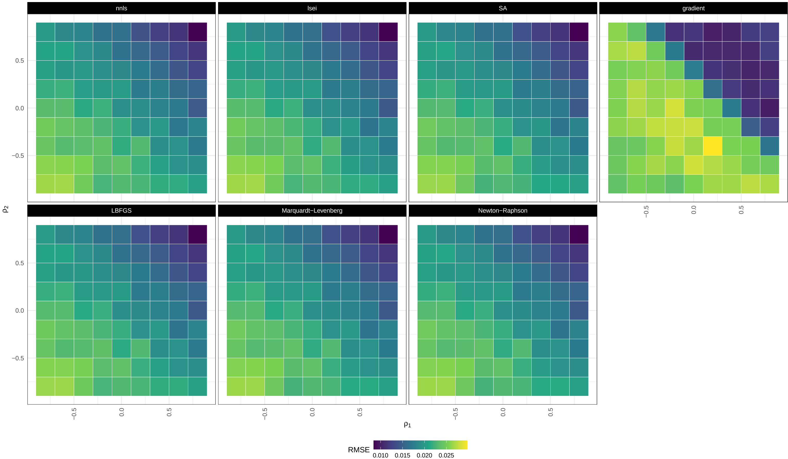
RMSE / large_CLD / homoscedastic / balanced
