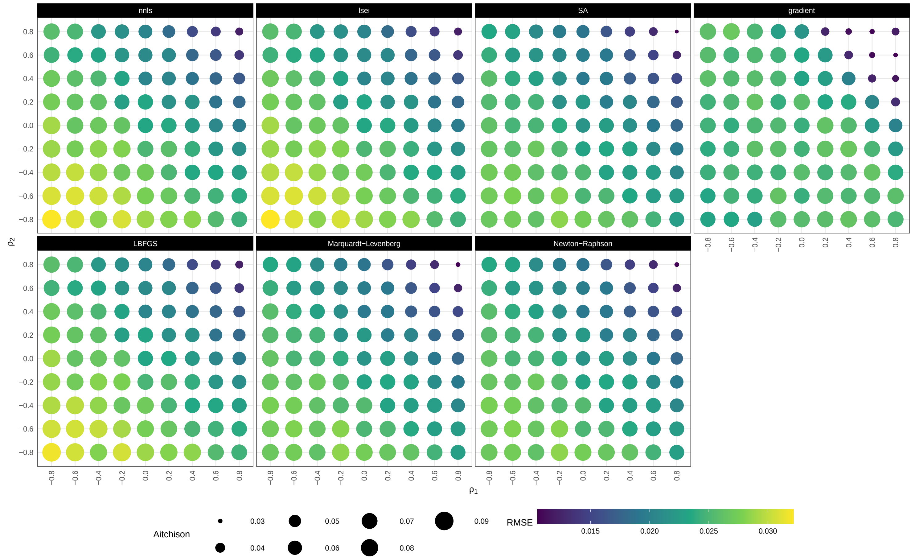
Each panel is the 9-by-9 correlation factorial (81 cells). Colour: mean RMSE; size: mean Aitchison distance.
