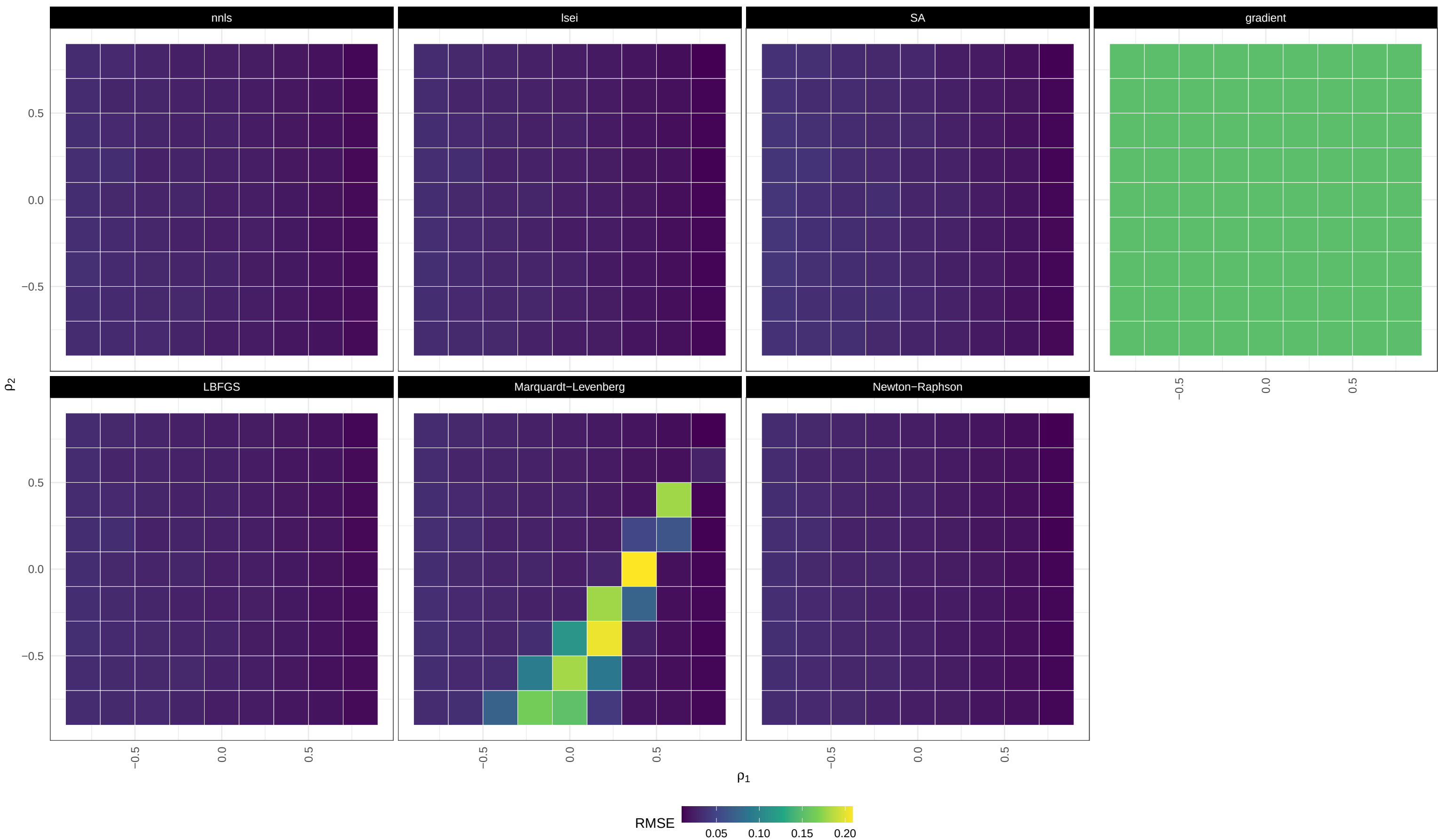
MAE / large_CLD / homoscedastic / moderately unbalanced
