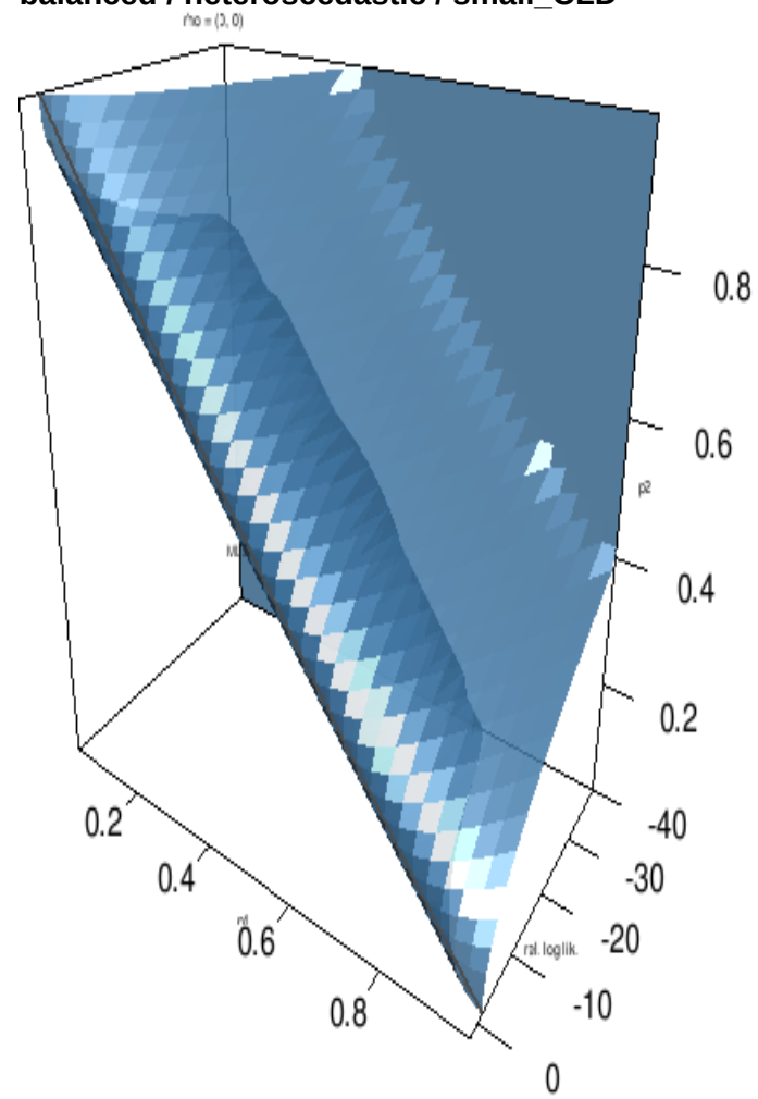
balanced / heteroscedastic / small_CLD
