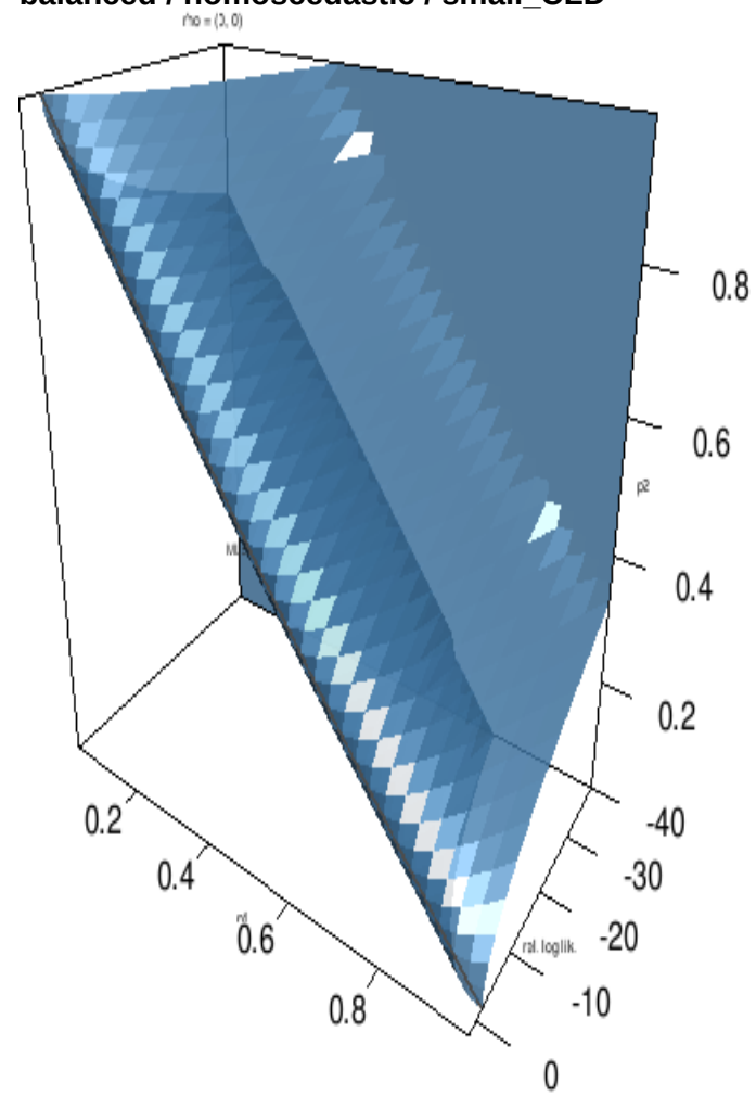
balanced / homoscedastic / small_CLD
