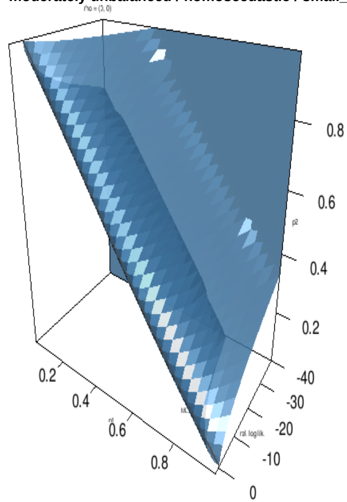
moderately unbalanced / homoscedastic / small_CLD
