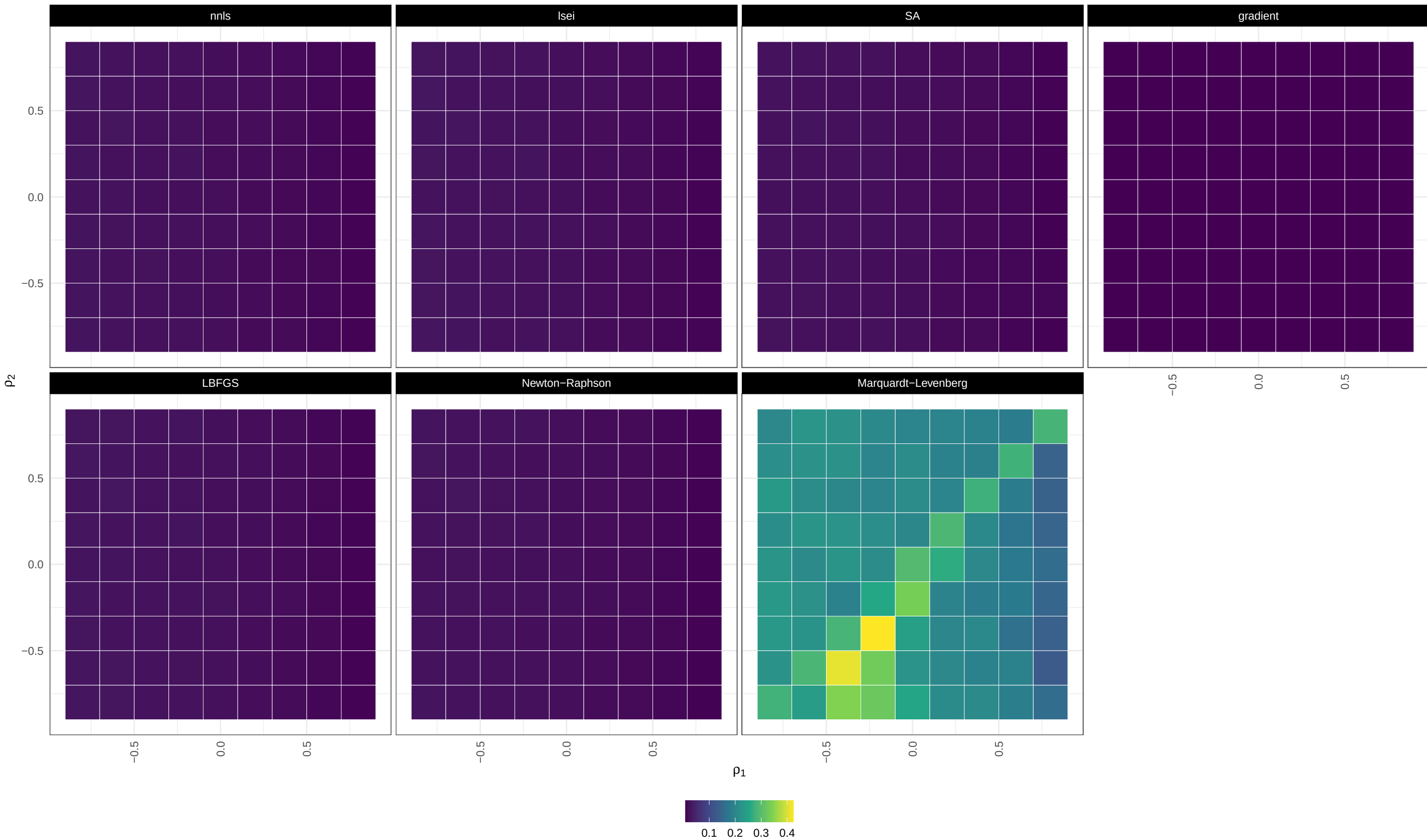
MAE / highly unbalanced / heteroscedastic / large_CLD
