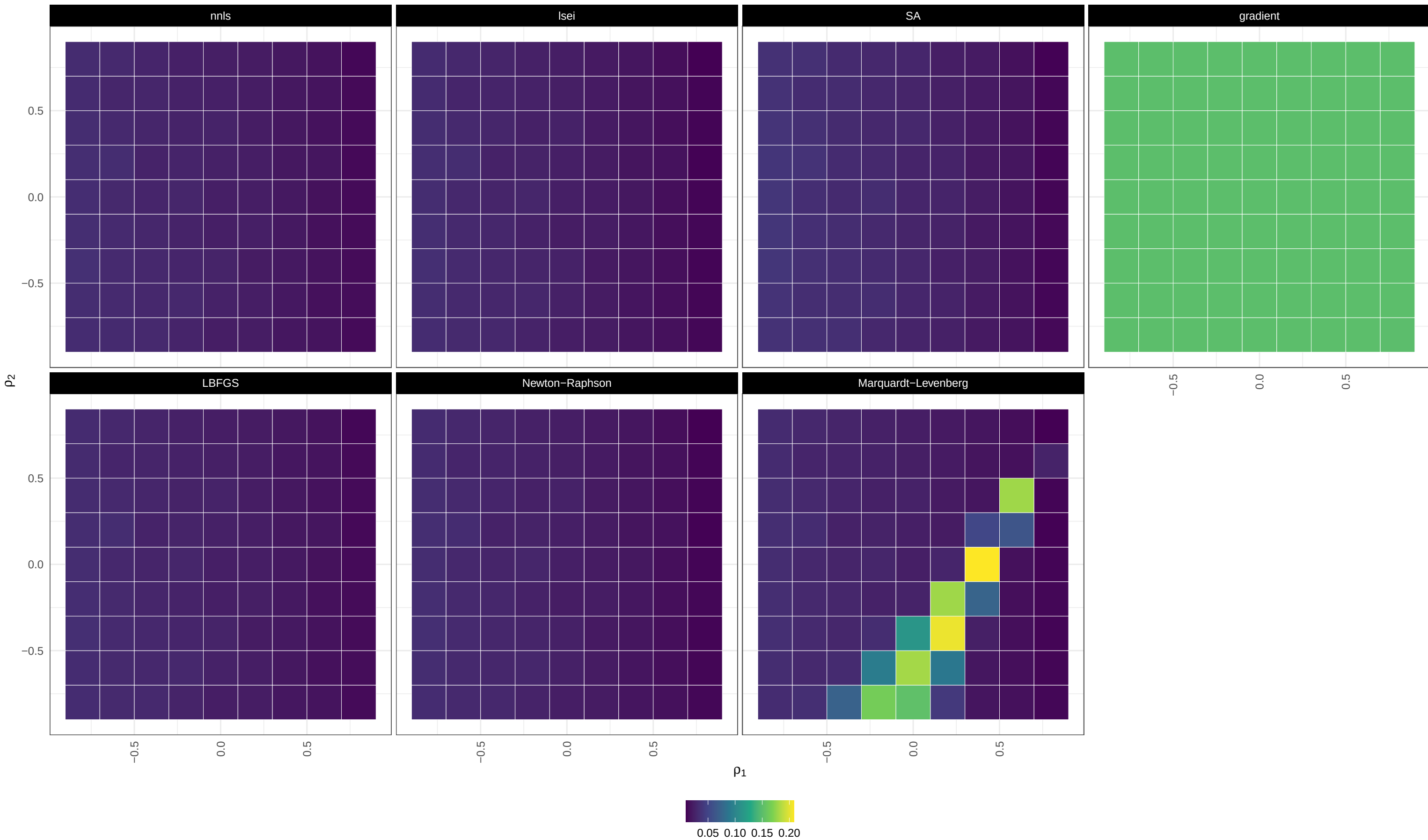
MAE / moderately unbalanced / homoscedastic / large_CLD
