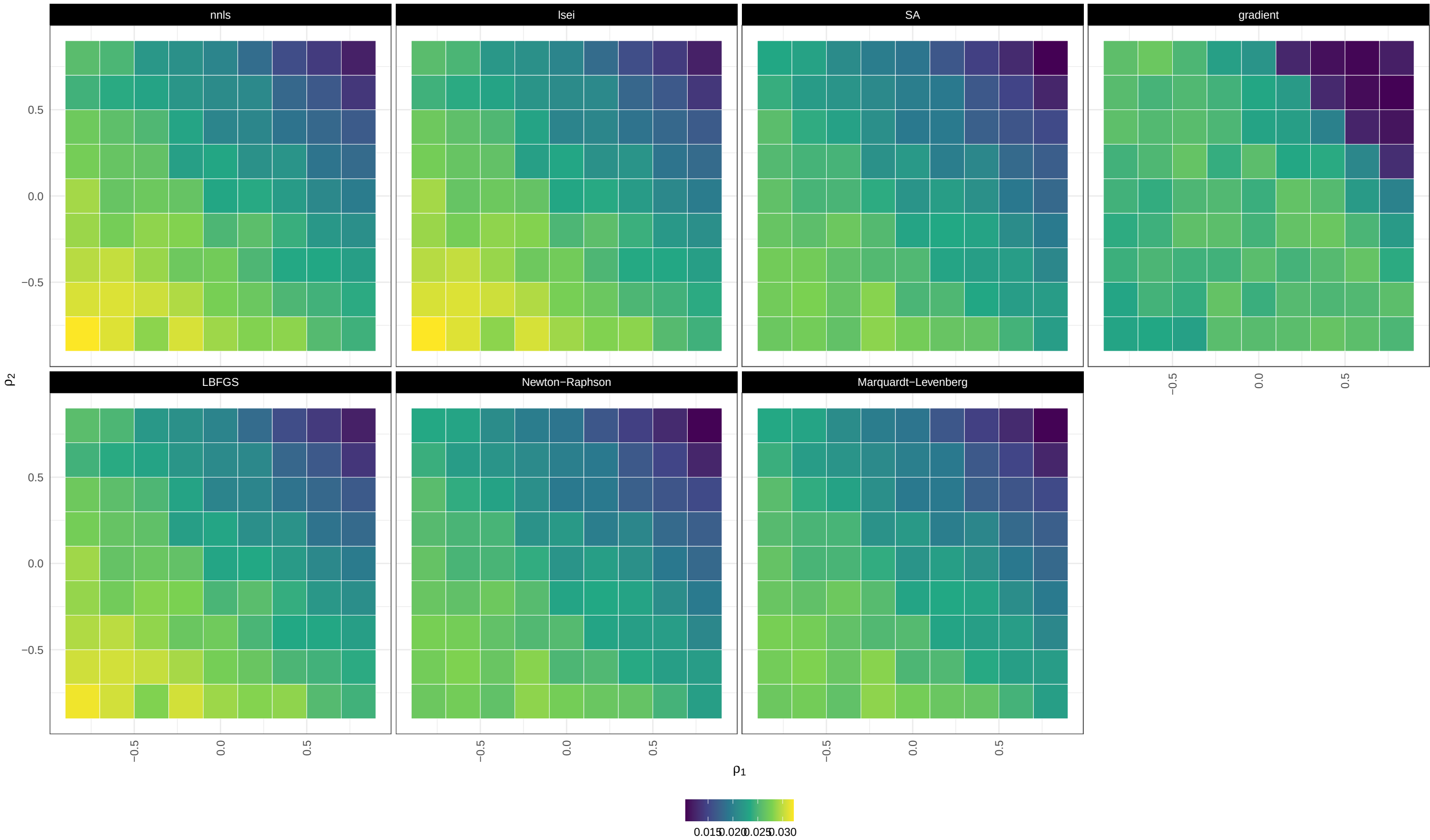
MAE / balanced / heteroscedastic / large_CLD
