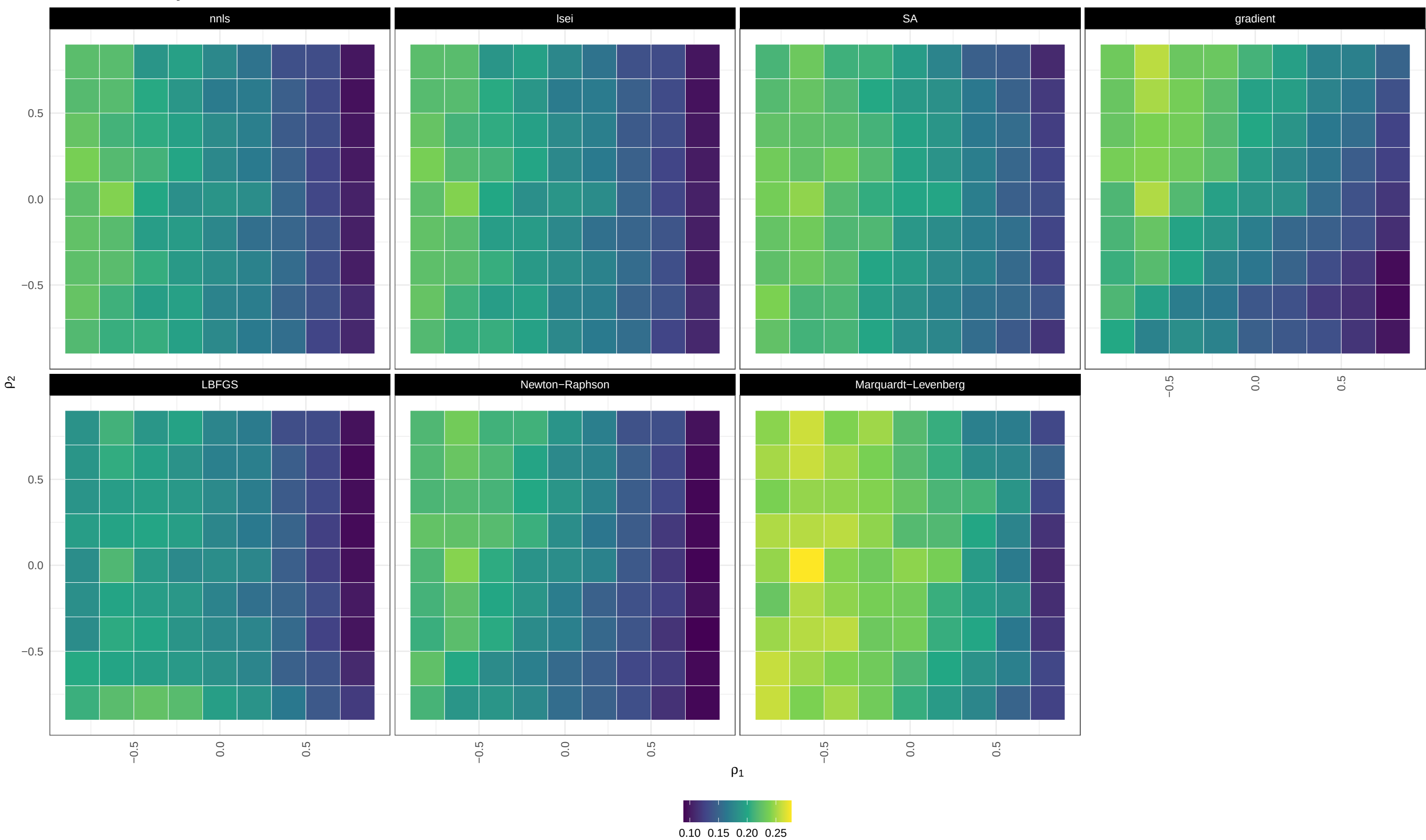
MAE / moderately unbalanced / homoscedastic / small_CLD
