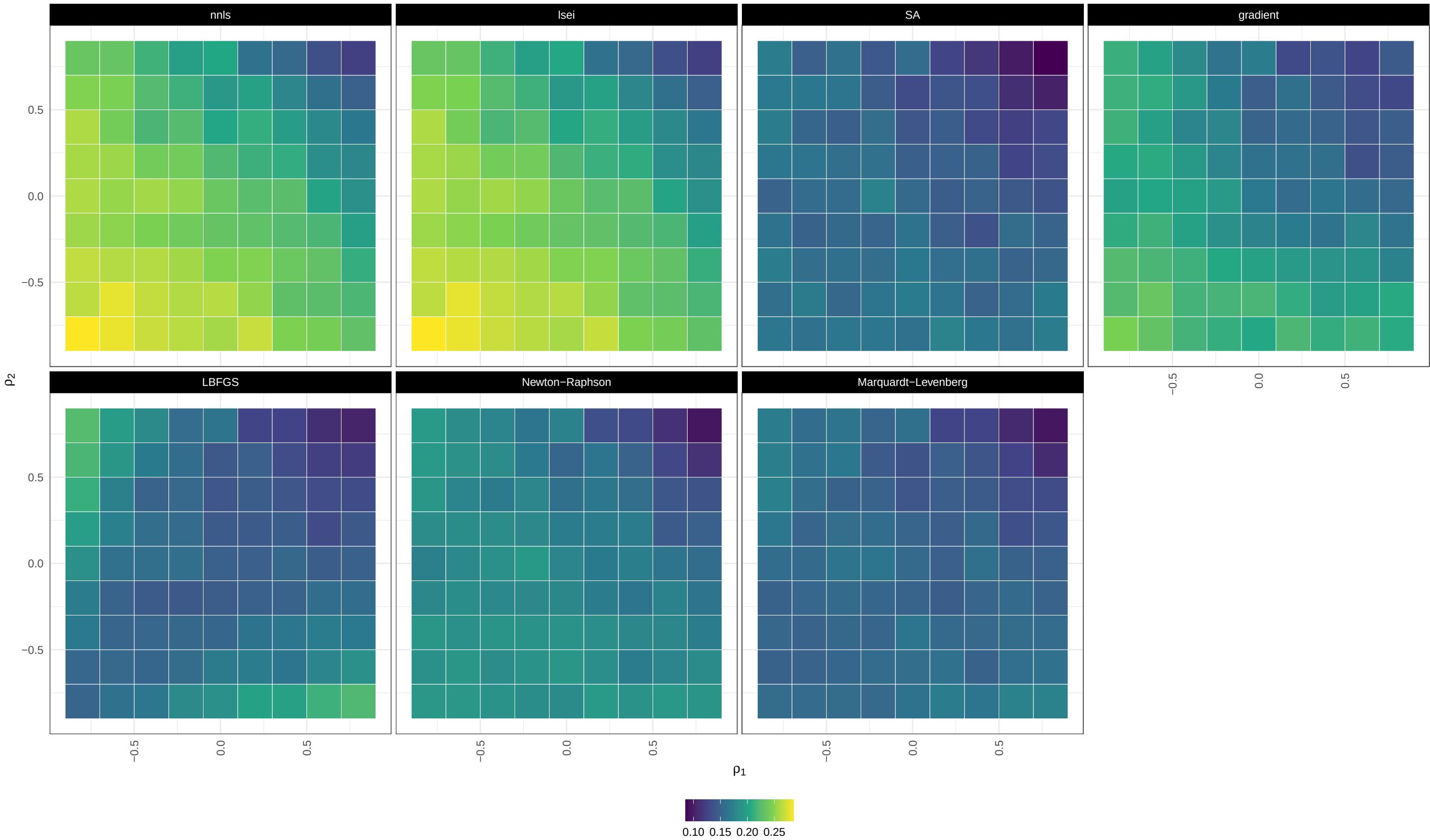
MAE / balanced / heteroscedastic / small_CLD
