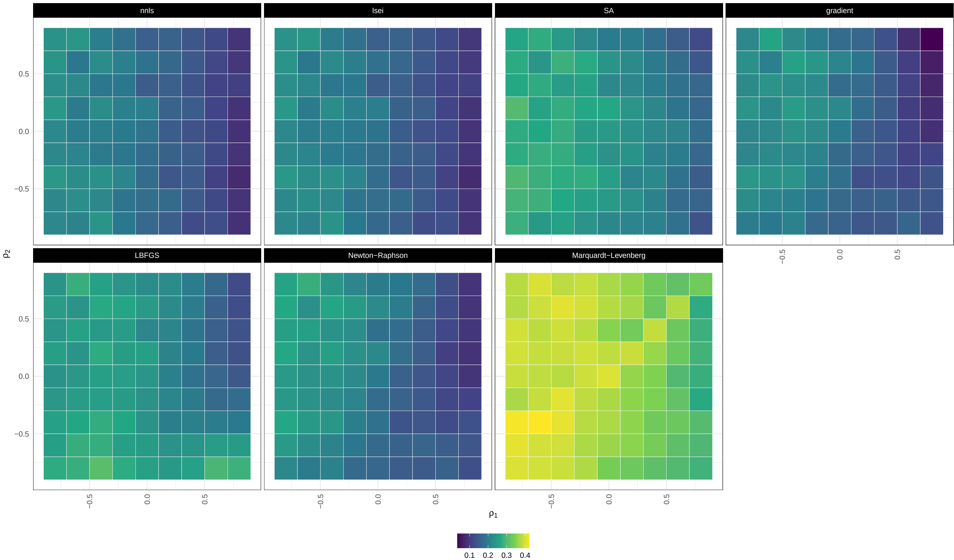
MAE / highly unbalanced / heteroscedastic / small_CLD
