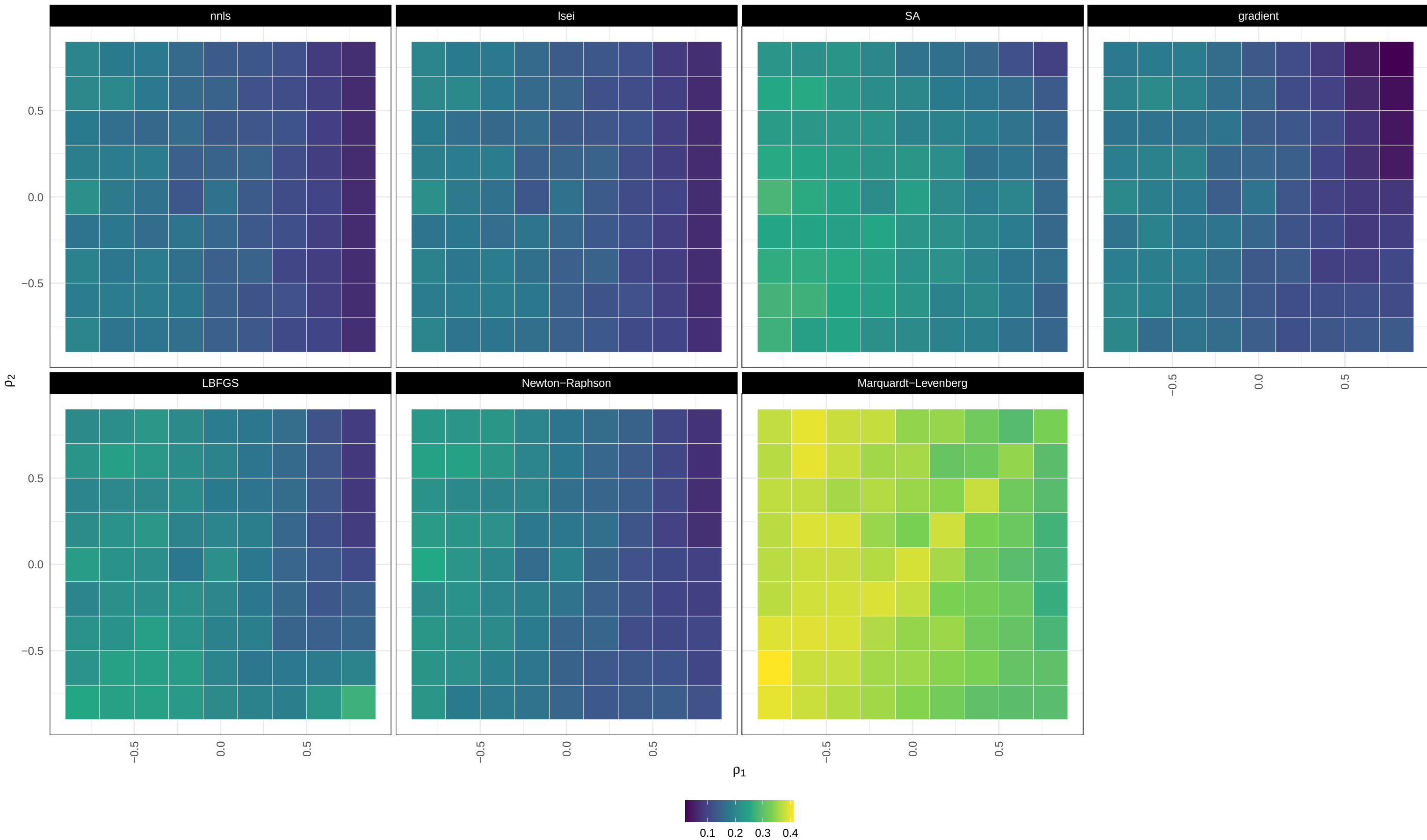
MAE / highly unbalanced / homoscedastic / small_CLD
