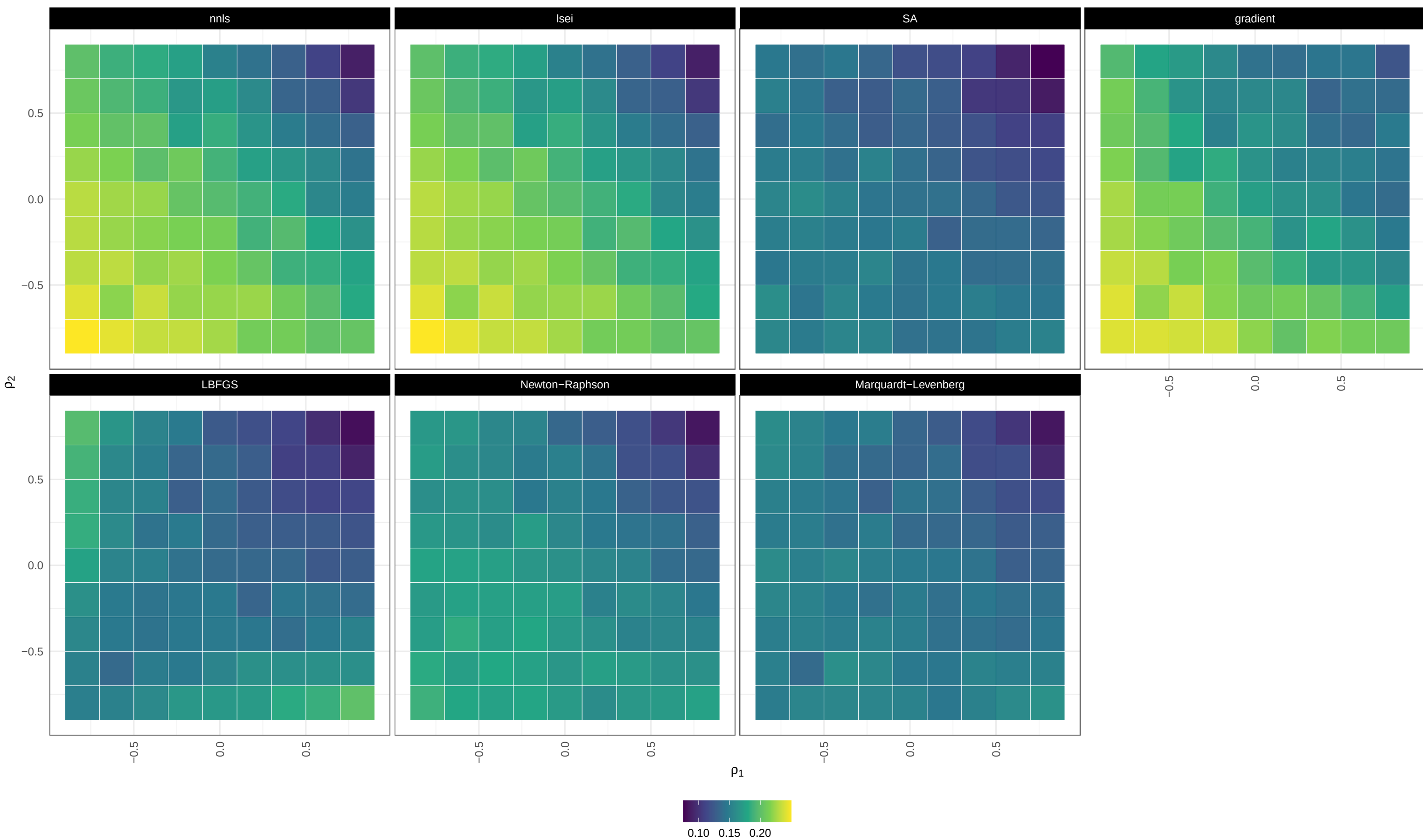
MAE / balanced / homoscedastic / small_CLD
