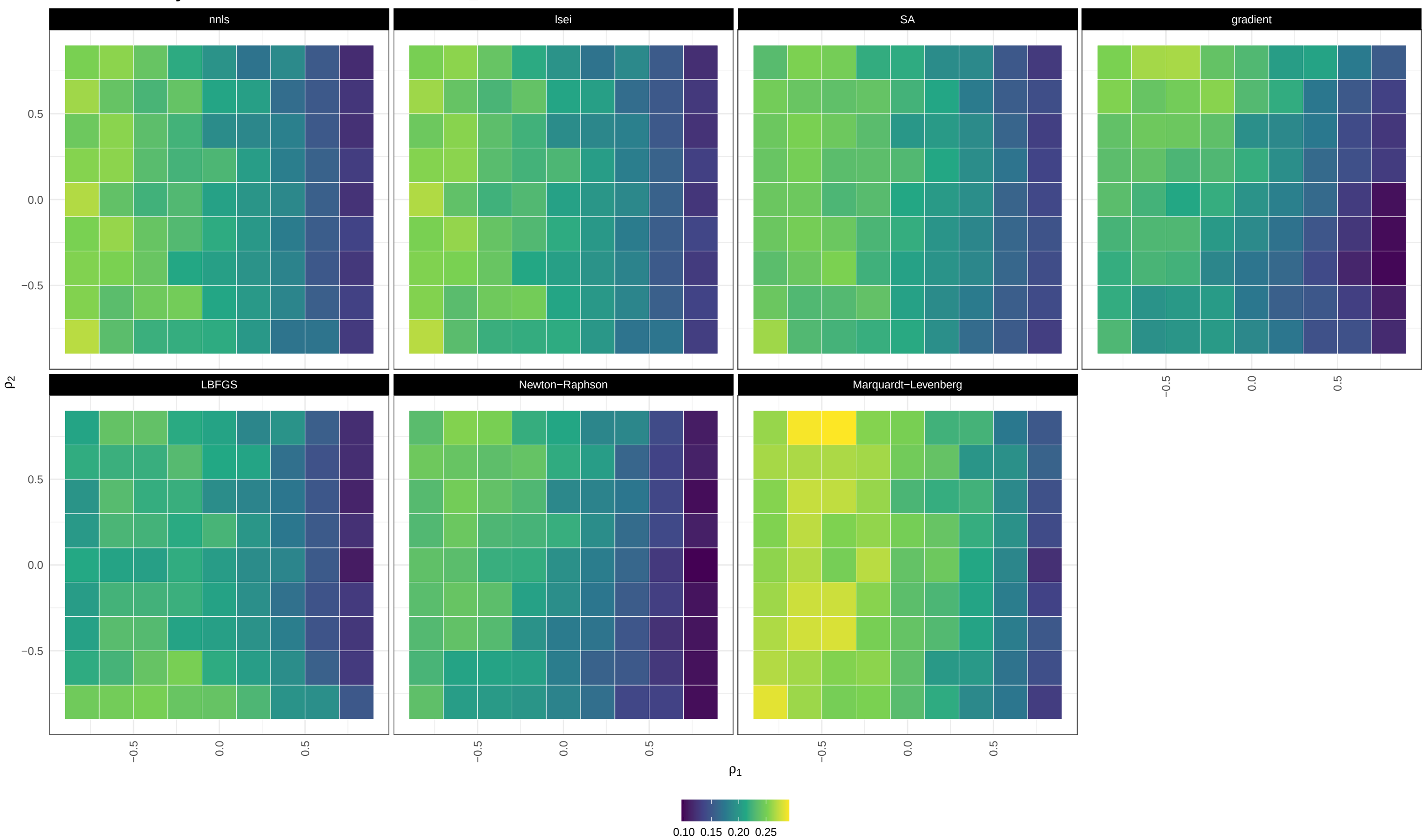
MAE / moderately unbalanced / heteroscedastic / small_CLD
