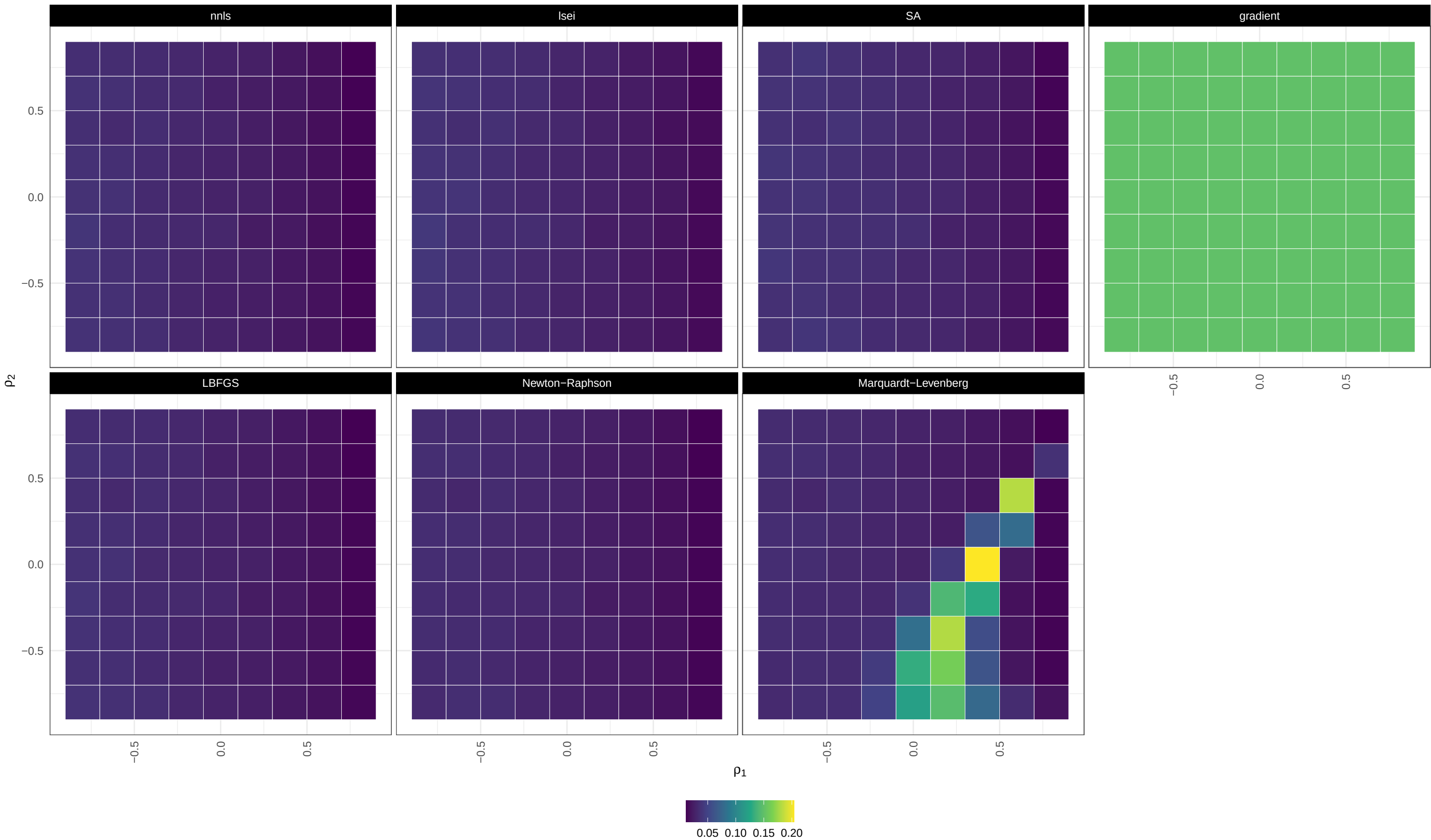
MAE / moderately unbalanced / heteroscedastic / large_CLD
