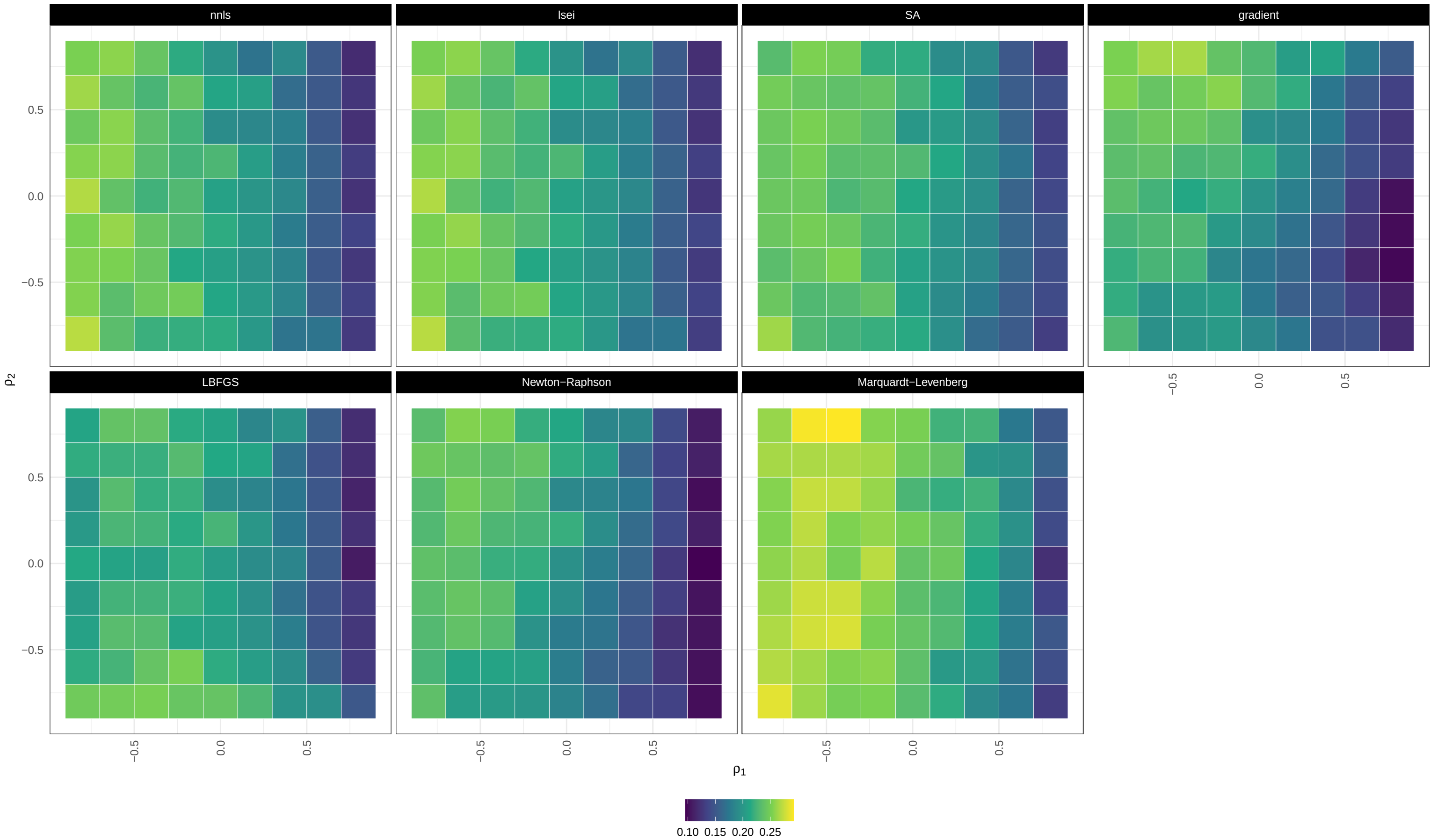
RMSE / moderately unbalanced / heteroscedastic / small_CLD
