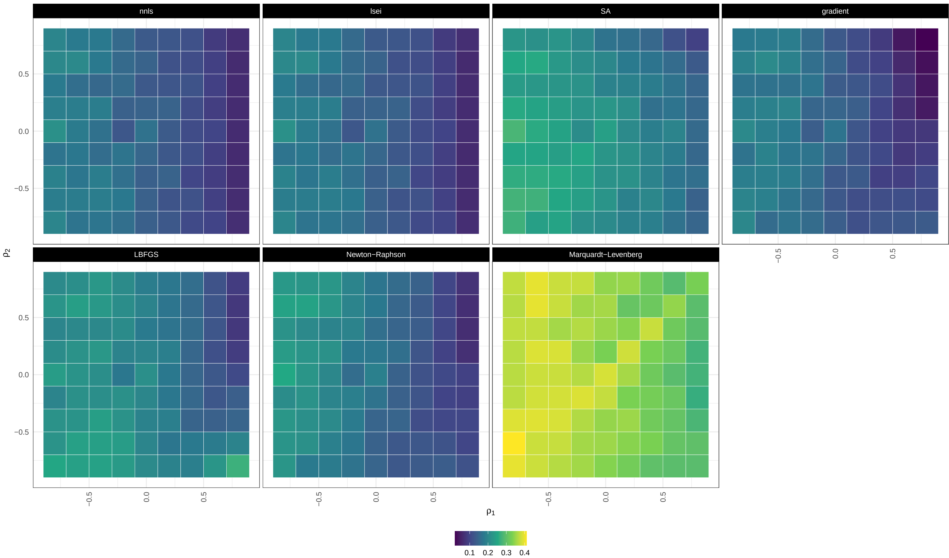
RMSE / highly unbalanced / homoscedastic / small_CLD
