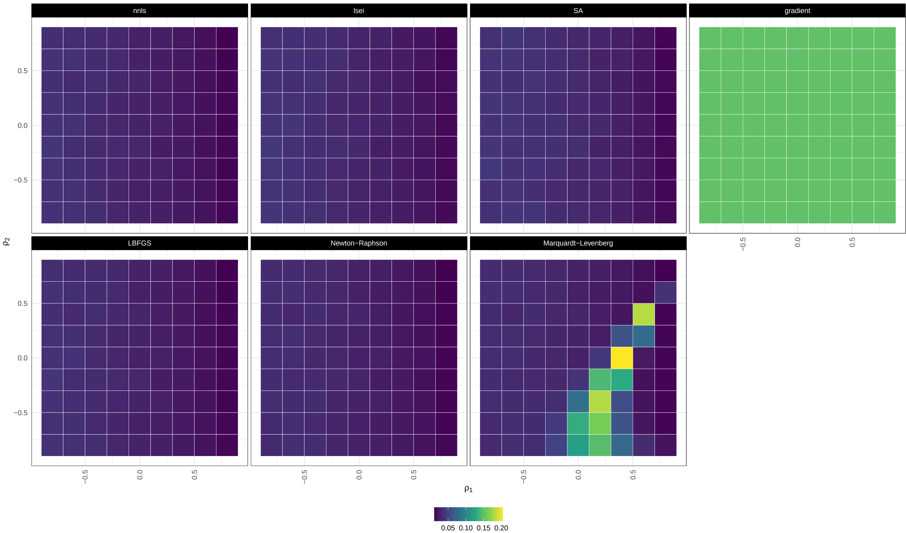
RMSE / moderately unbalanced / heteroscedastic / large_CLD
