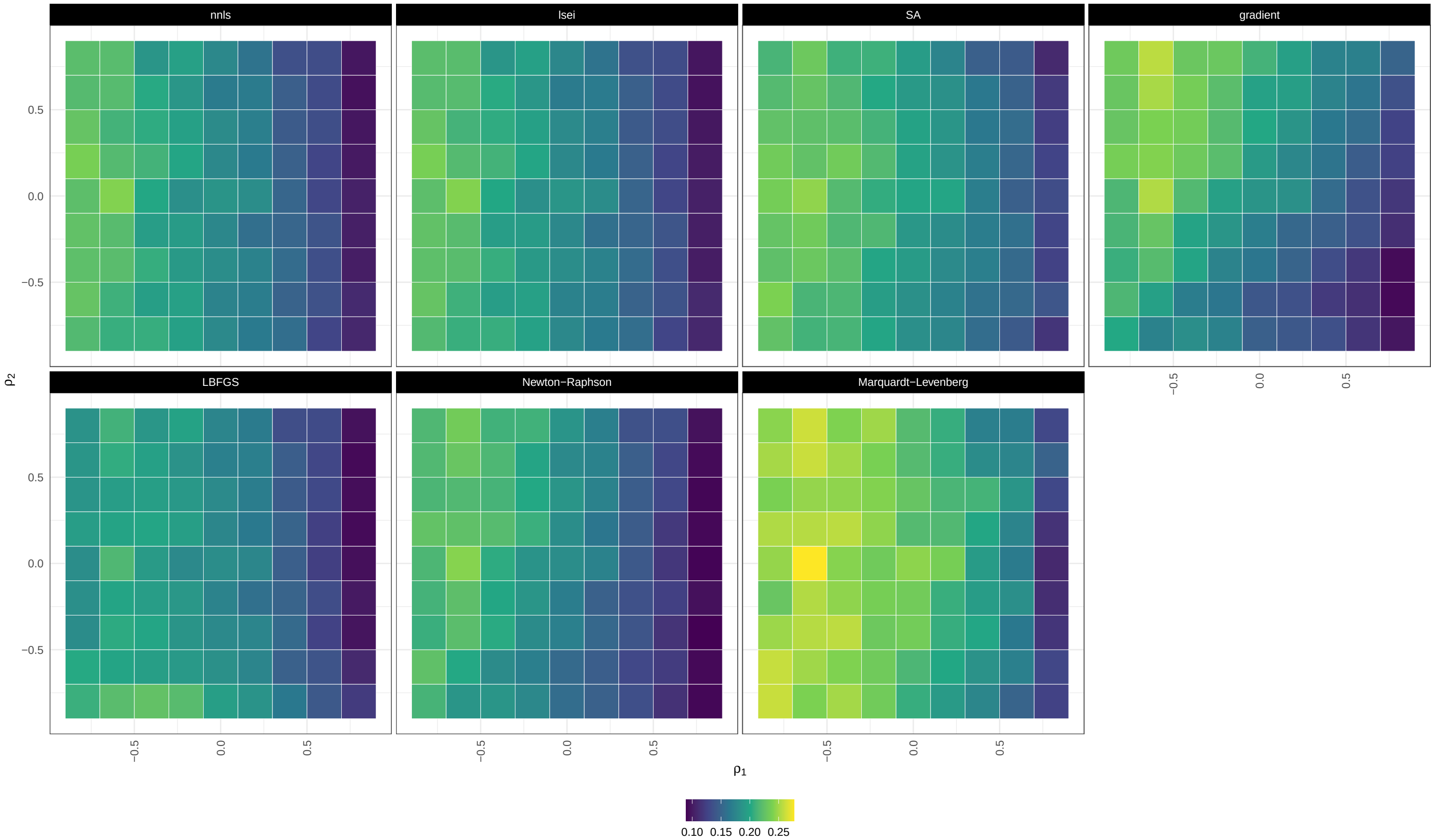
RMSE / moderately unbalanced / homoscedastic / small_CLD
