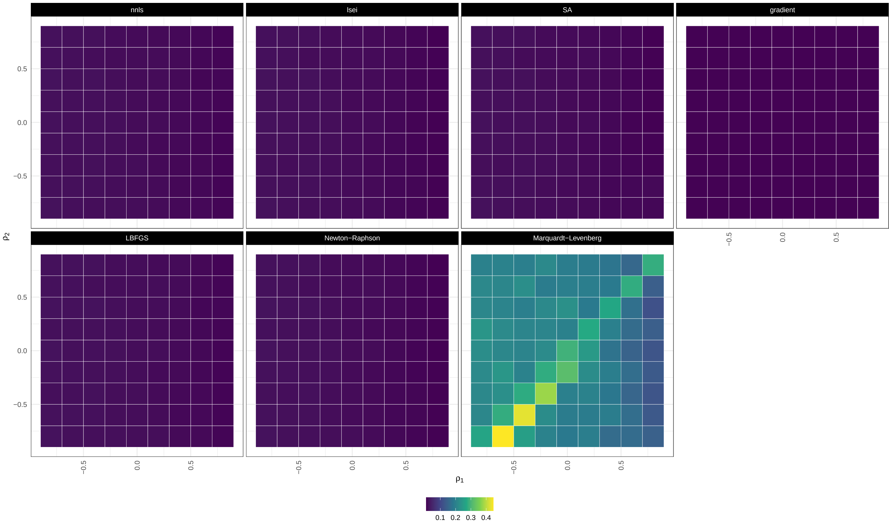
RMSE / highly unbalanced / homoscedastic / large_CLD
