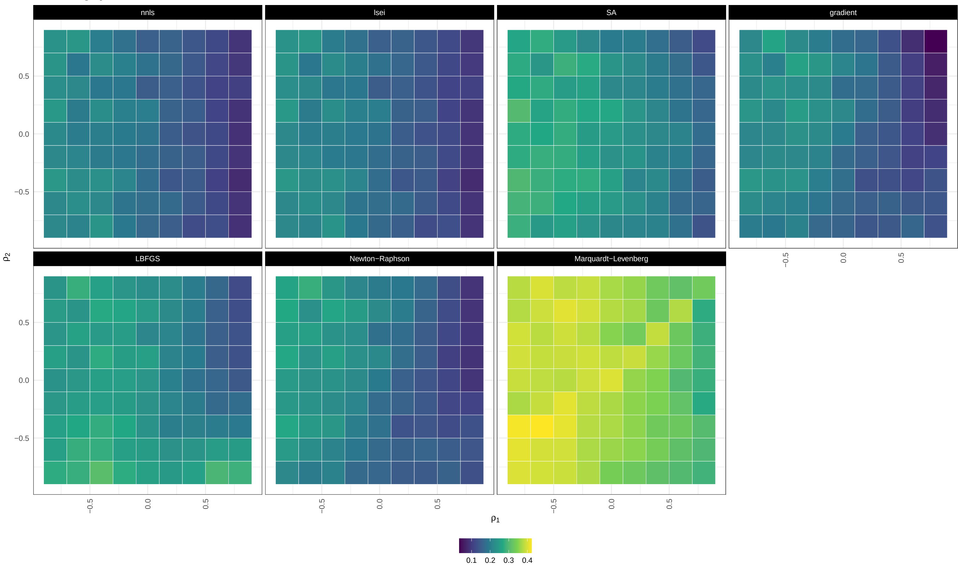
RMSE / highly unbalanced / heteroscedastic / small_CLD
