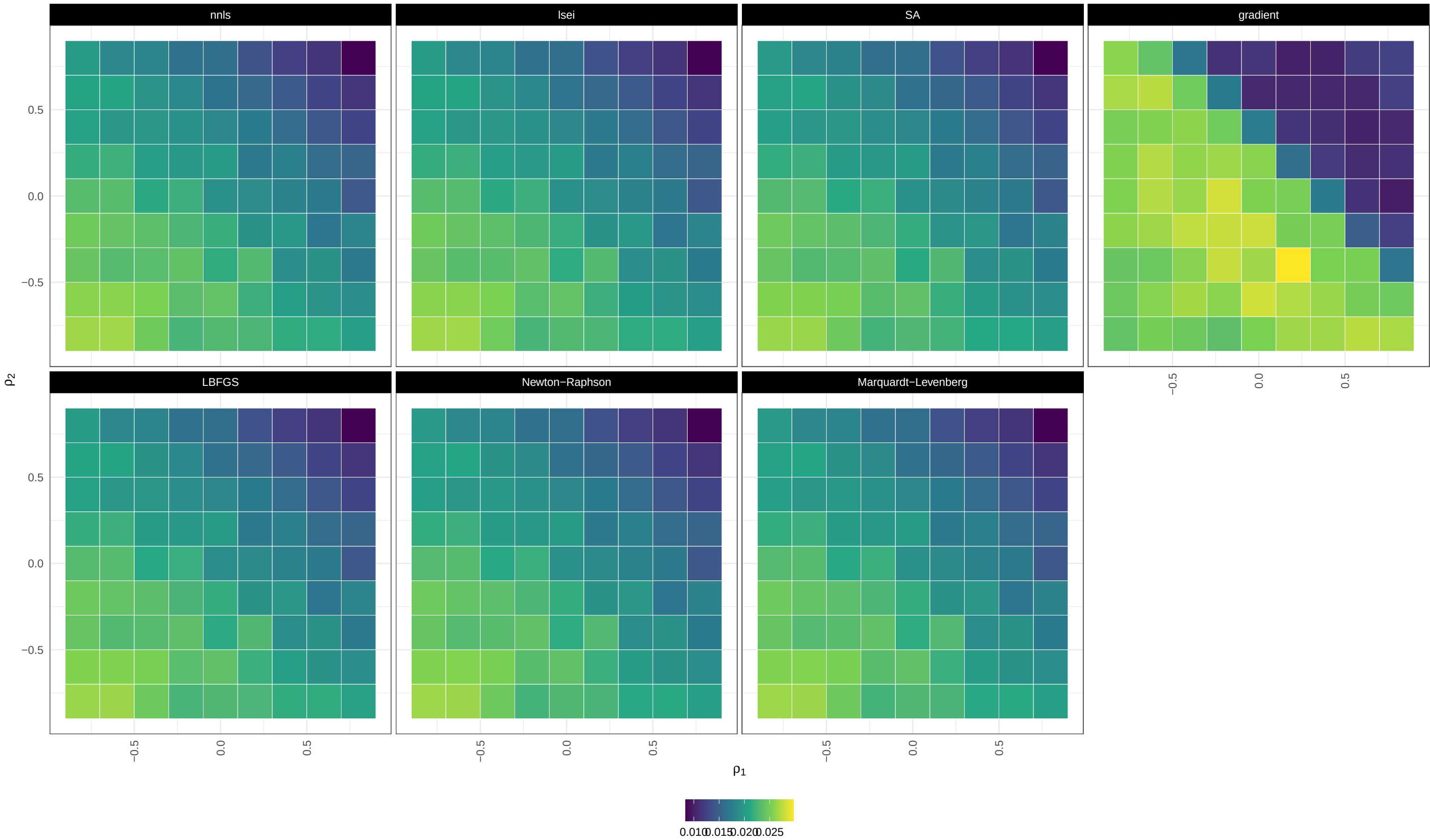
RMSE / balanced / homoscedastic / large_CLD
