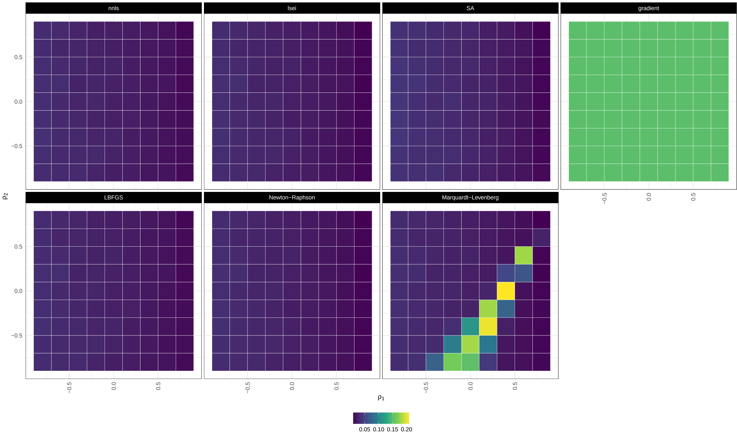
RMSE / moderately unbalanced / homoscedastic / large_CLD
