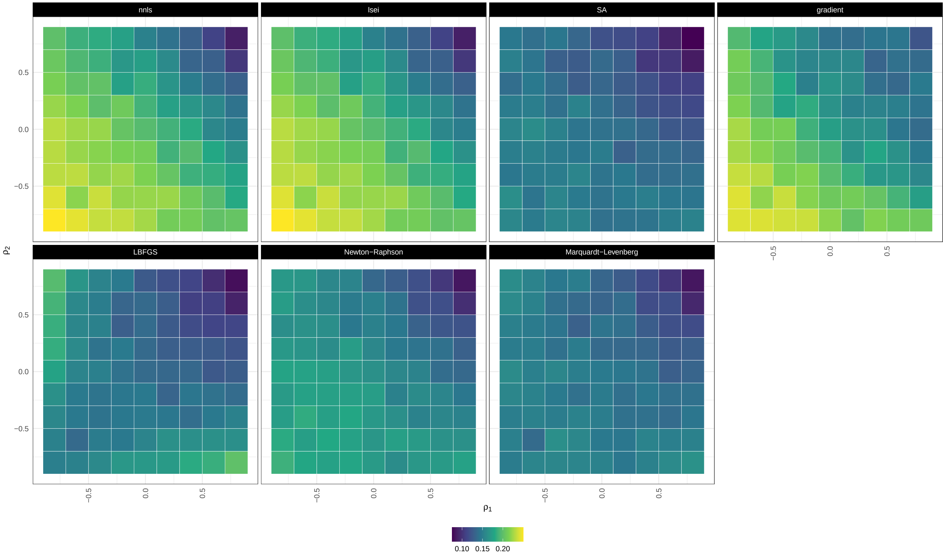
RMSE / balanced / homoscedastic / small_CLD
