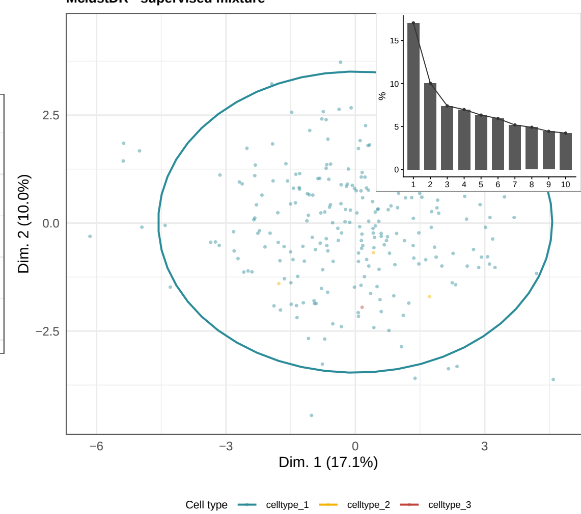
F MclustDR · supervised mixture
