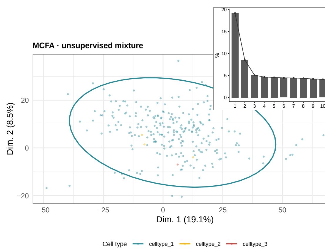
E MCFA · unsupervised mixture
