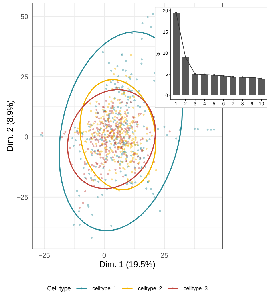
D MCFA · convolution
