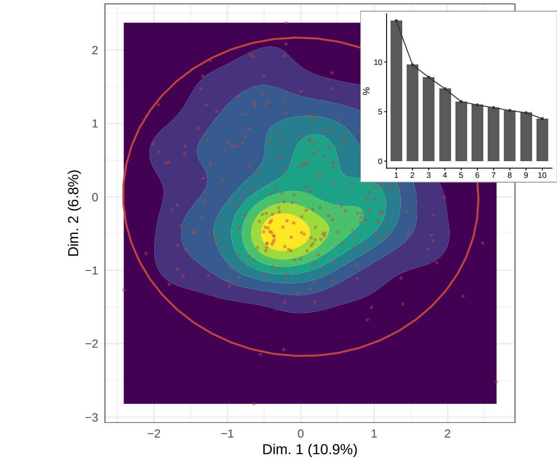
C celltype_3 · Thomson FA
