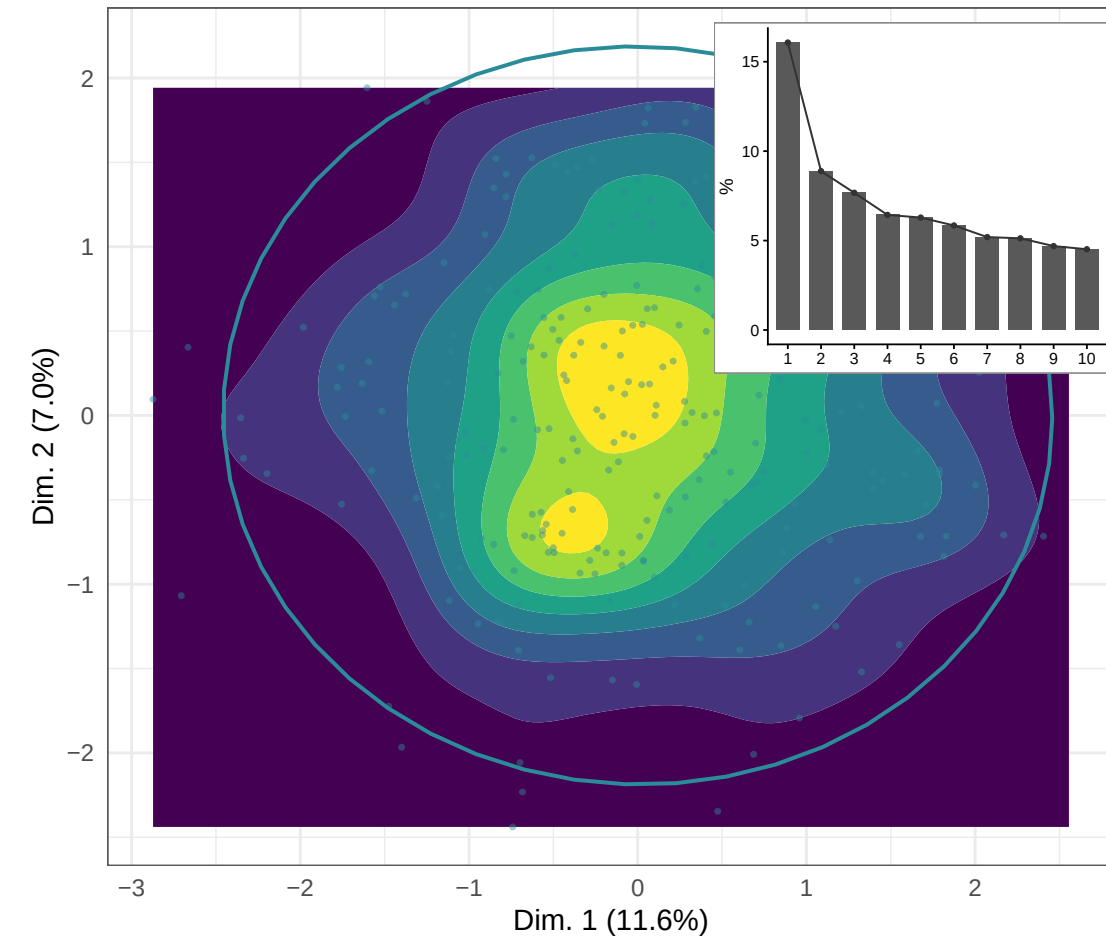
A celltype_1 · Thomson FA
