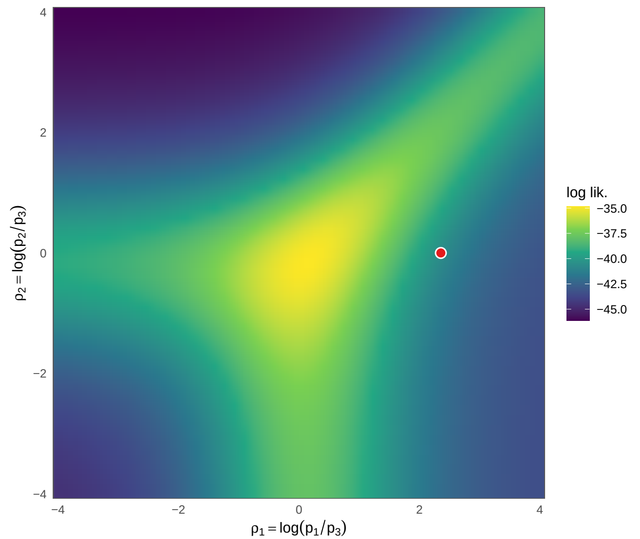
CT1 Cluster SBM / CT2 Cluster SBM
