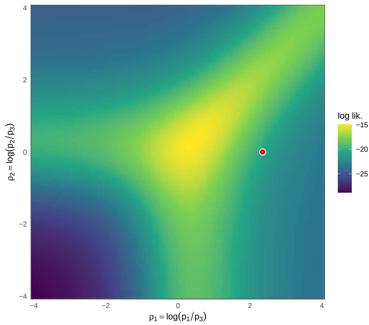
CT1 Cluster SBM / CT2 Cluster SBM
