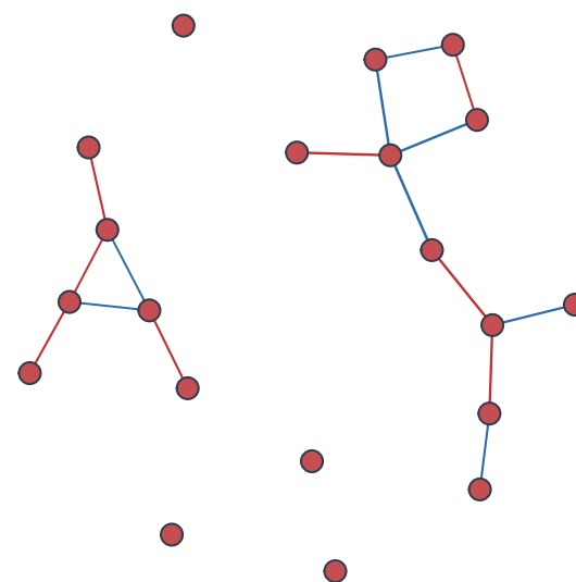
CT2 Cluster SBM
