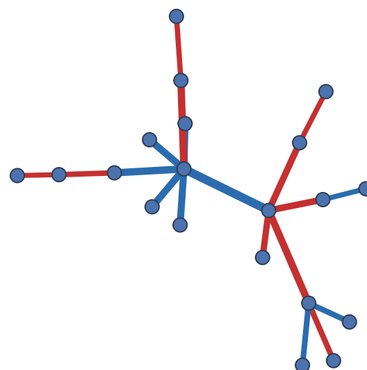
CT1 Cluster SBM
