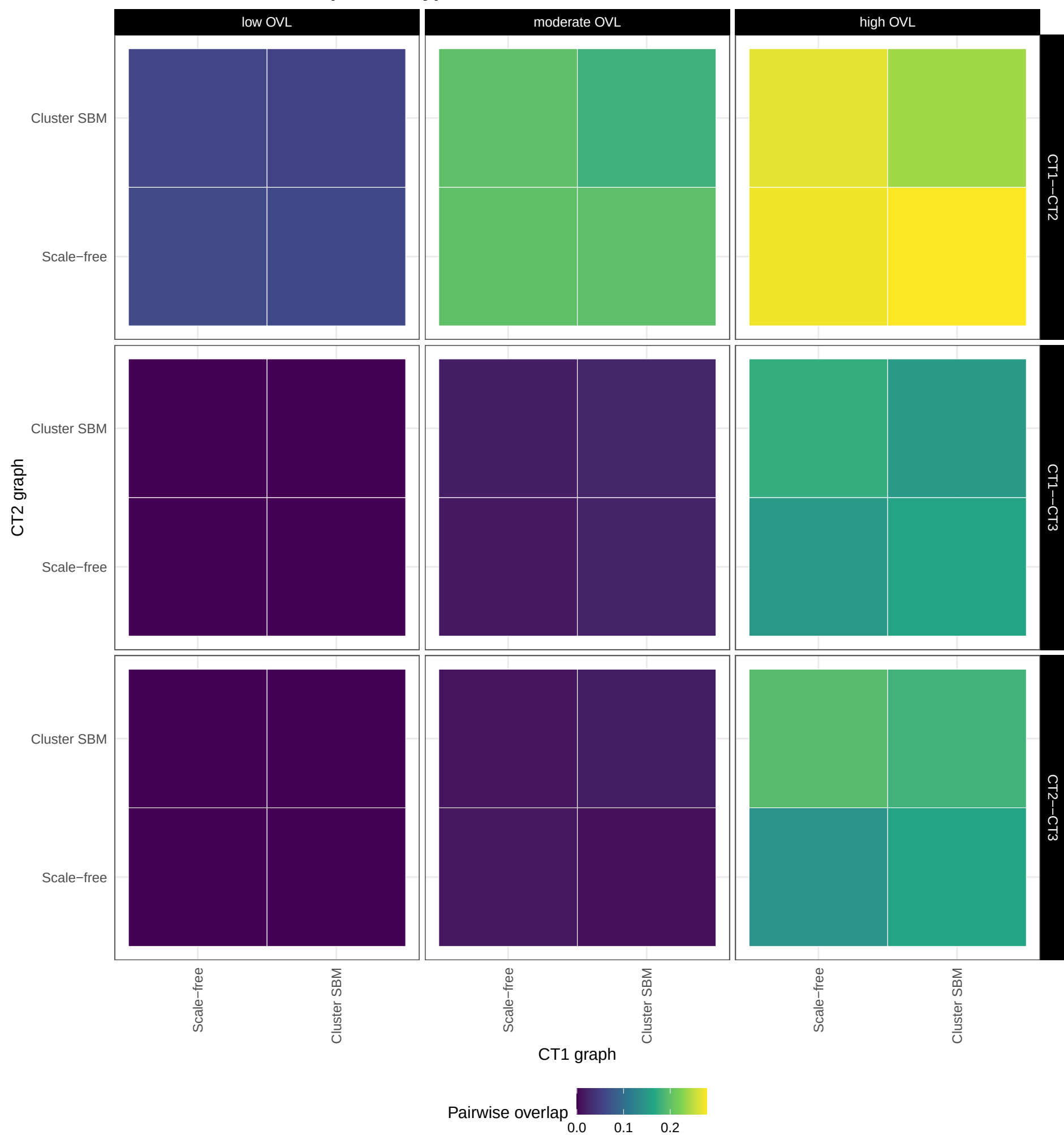
Pairwise MixSim overlap of cell-type Gaussians
