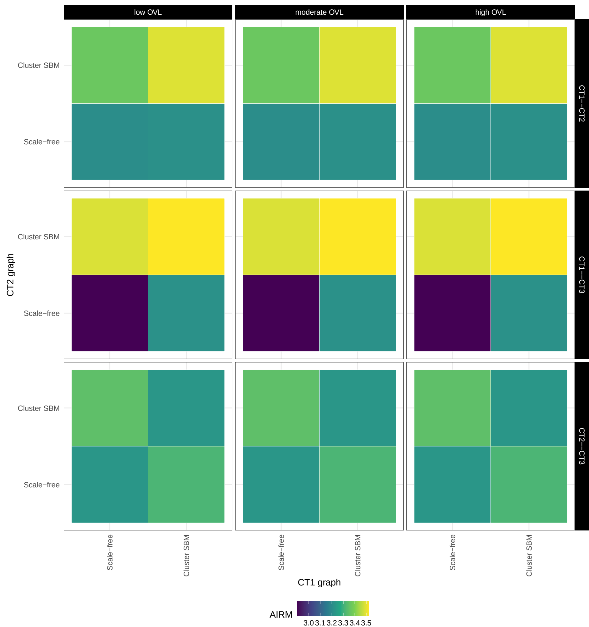
Pairwise affine-invariant Riemannian distance of Sigma_j
