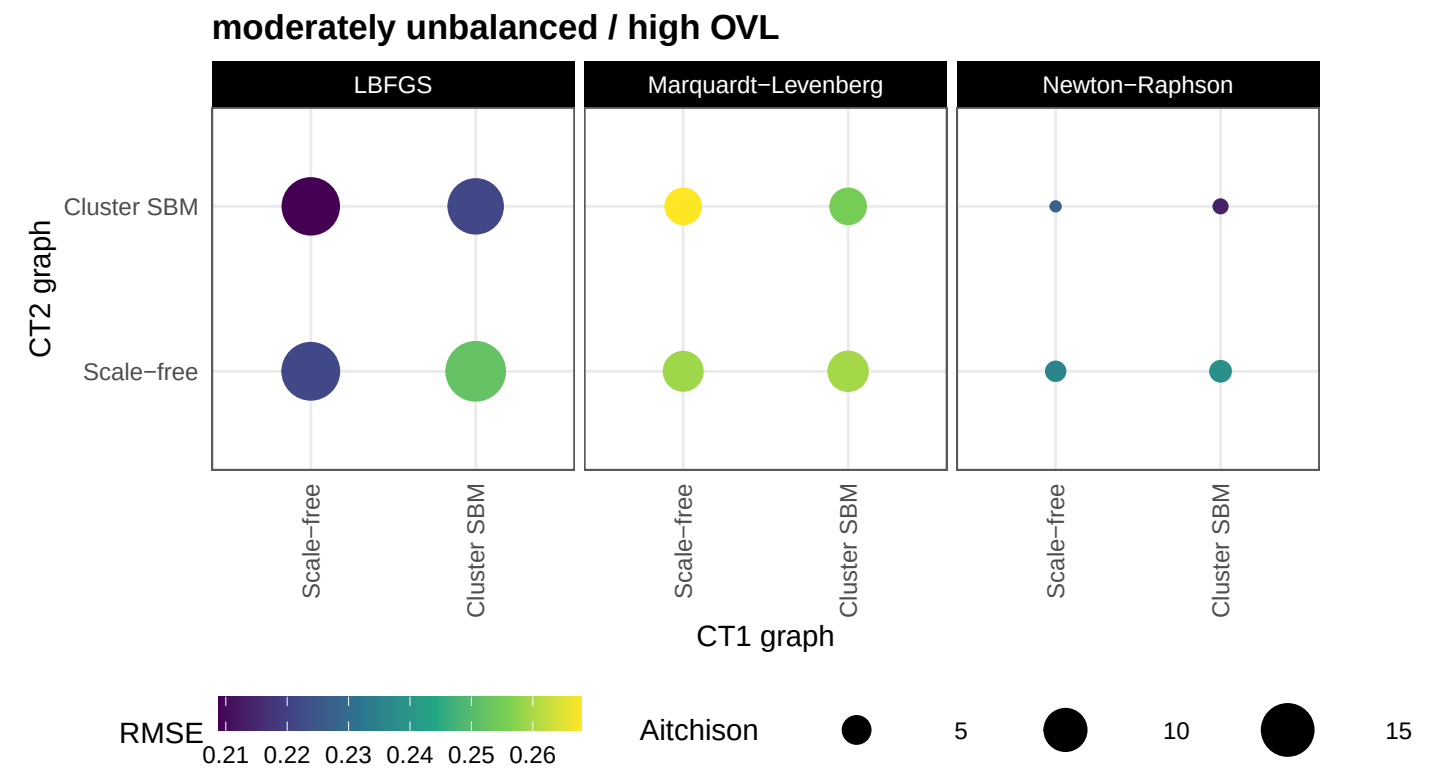
Each panel is the 2-by-2 of CT1 / CT2 graph families. Colour: mean RMSE; size: mean Aitchison distance.
