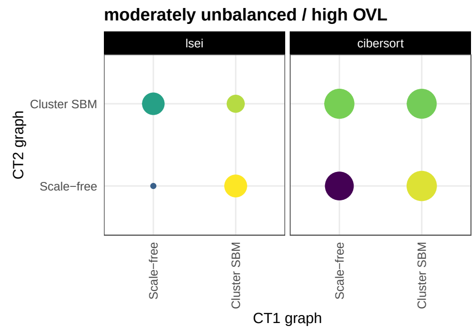
Each panel is the 2-by-2 of CT1 / CT2 graph families. Colour: mean RMSE; size: mean Aitchison distance.
