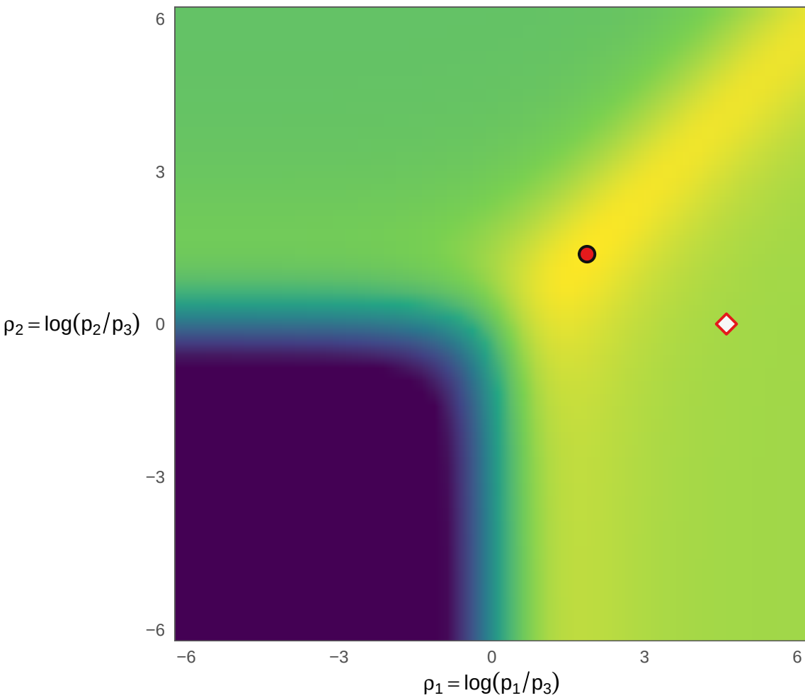
CT1 Scale-free / CT2 Scale-free
