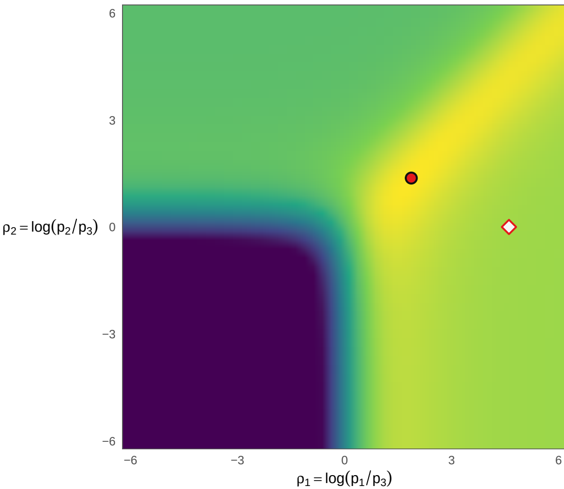
CT1 Cluster SBM / CT2 Scale-free
