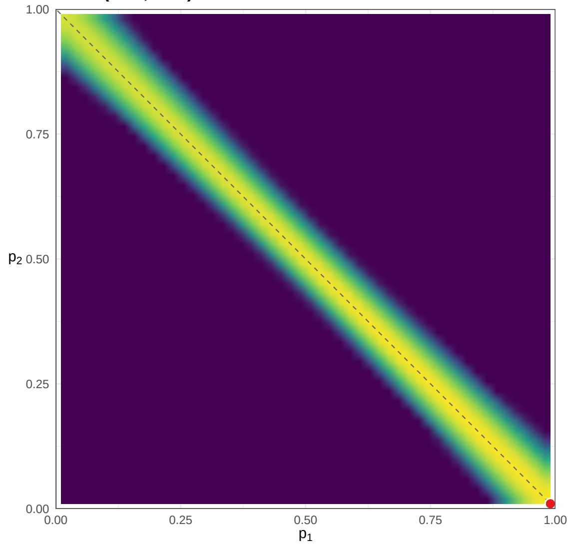
small_CLD / homoscedastic / highly unbalanced
