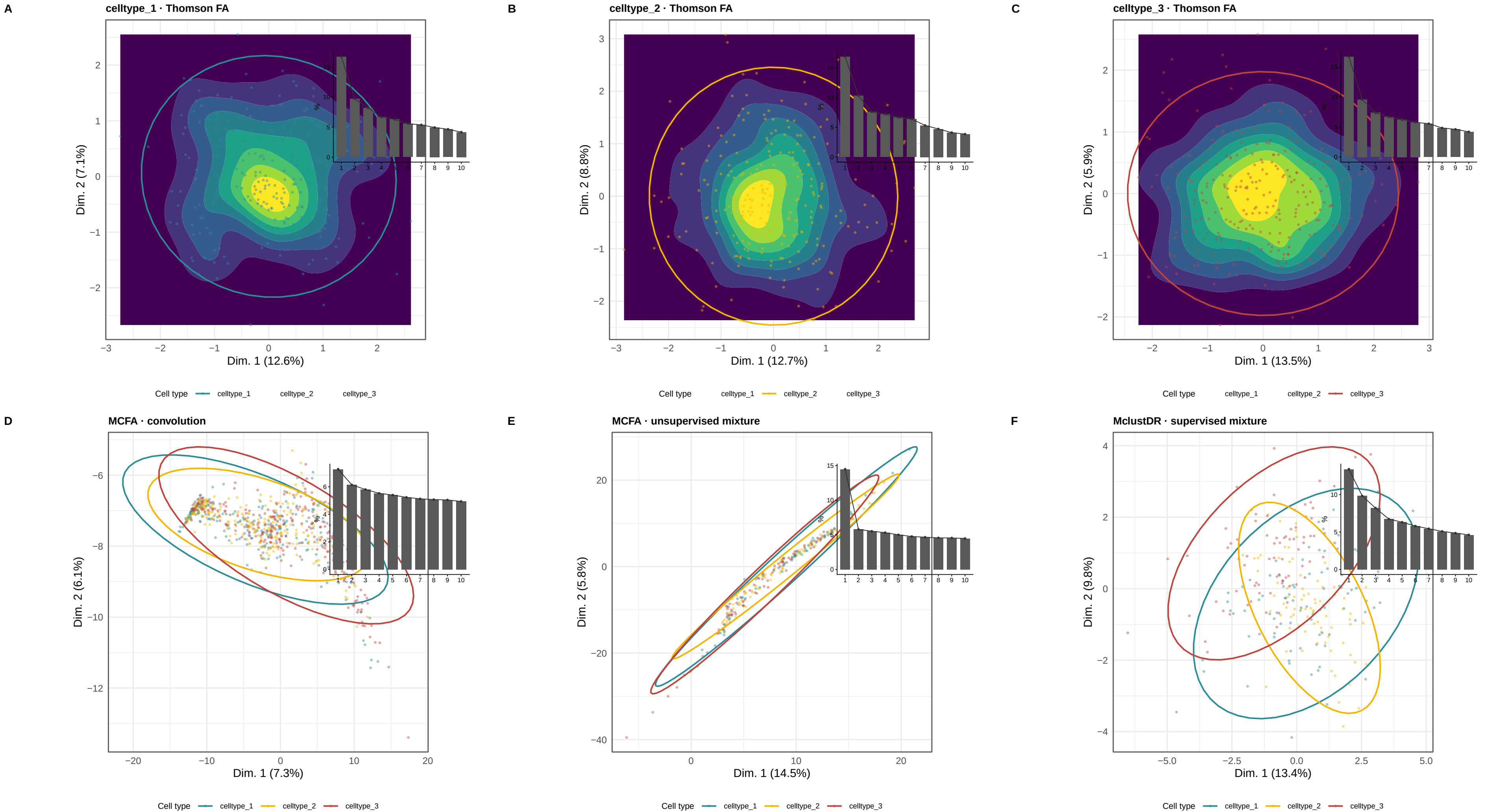
A: Independent Thomson factanal() on purified type 1 (regression scores). B: Independent Thomson factanal() on purified type 2 (regression scores). C: Independent Thomson factanal() on purified type 3 (regression scores). D: MCFA fitted to convolution bulk draws (weights p_j^2 ); purified slices scored in that plane. E: MCFA fitted to unsupervised mixture draws (one type per draw, weights p_j ). F: Supervised MclustDA (EDDA) then MclustDR on labelled mixture draws. Insets: first 10 eigenvalues.
