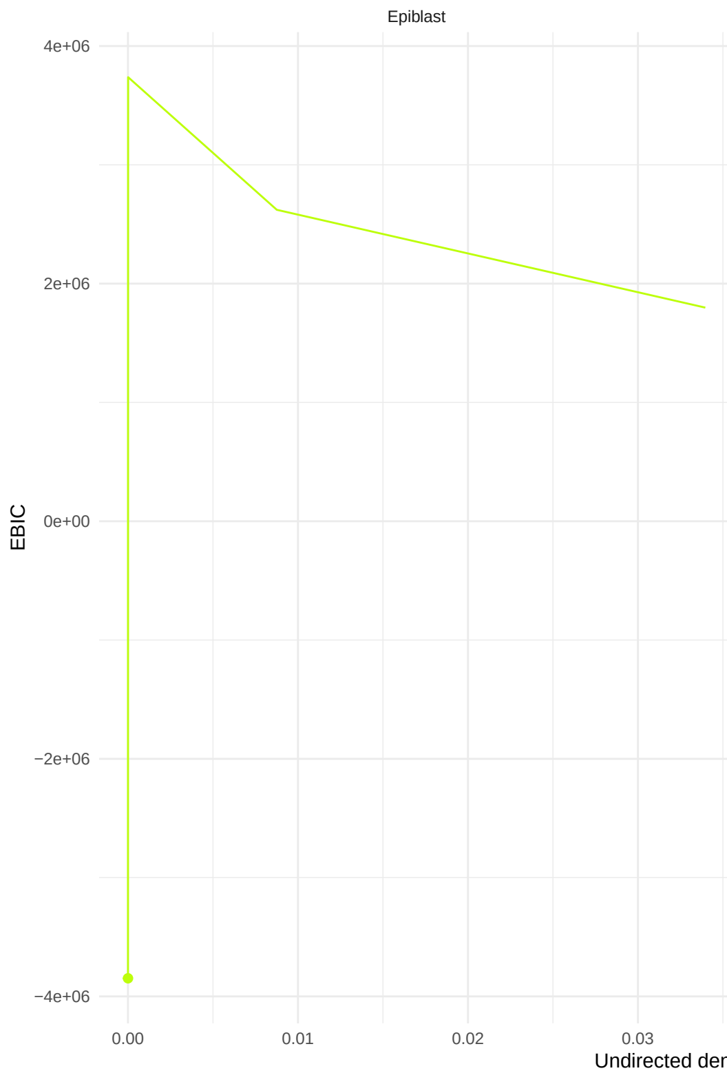
Edge density against EBIC, 48h
