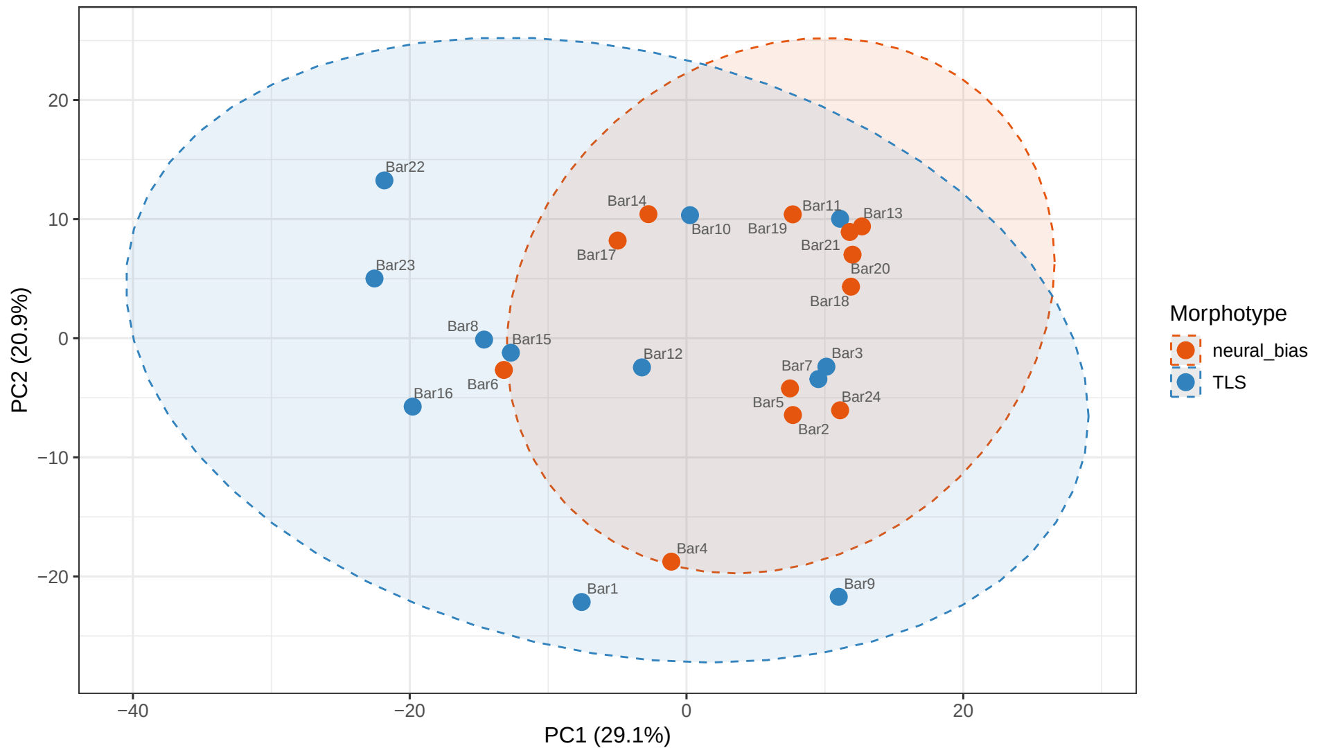
PCA – naive pseudo-bulk samples
