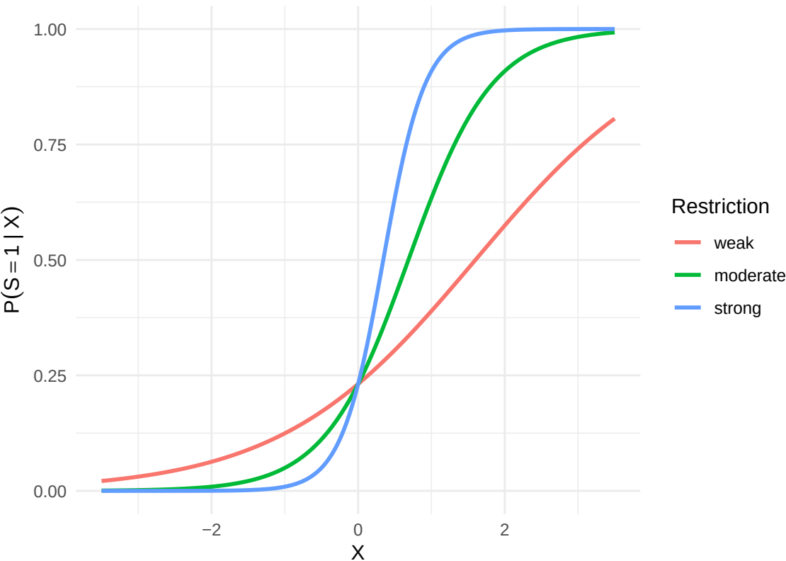
Logistic selection on continuous X
