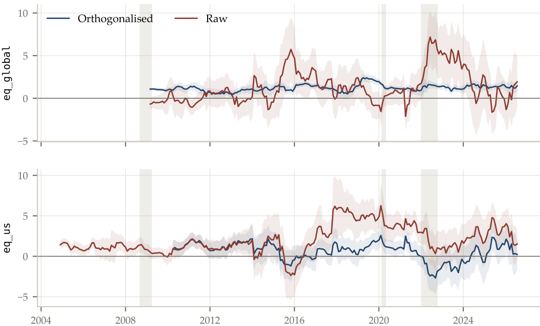
Beta paths with 95% HAC bands: what each panel calls 'equity exposure'
