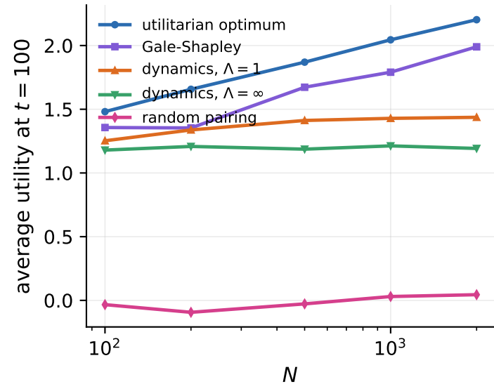
Gaussian model, \mathcal{N}(0, 1)
