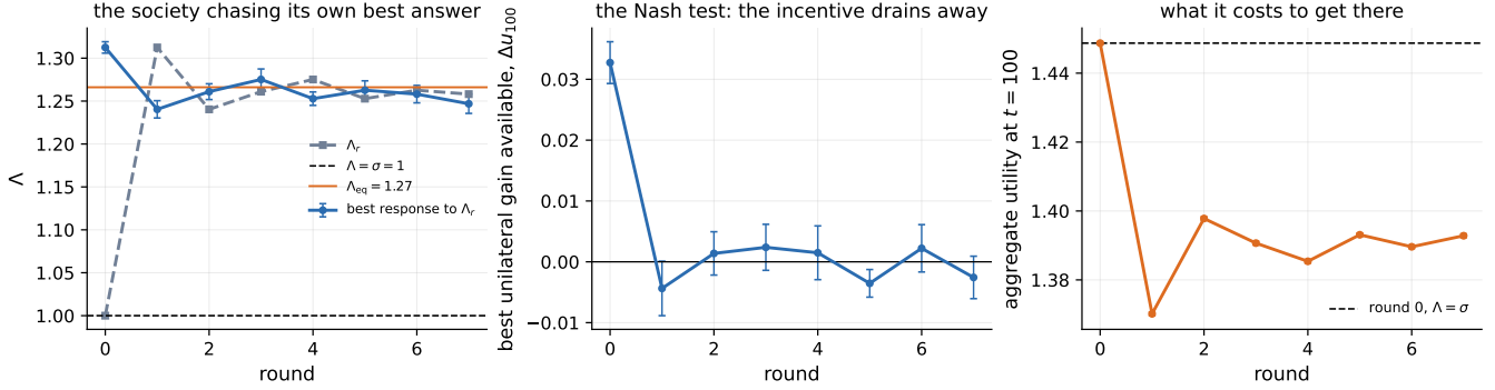
Figure 6: Iterated best response from the convention \Lambda = \sigma , Gaussian model, N = 10,000 , 256 societies per round. Left: the society chasing its own best answer. Centre: the best unilateral gain available, which is the Nash test — it is ten standard errors from zero at round 0 and statistically zero from round 1 on. Right: aggregate utility, which peaks at round 0 and can only fall thereafter.
