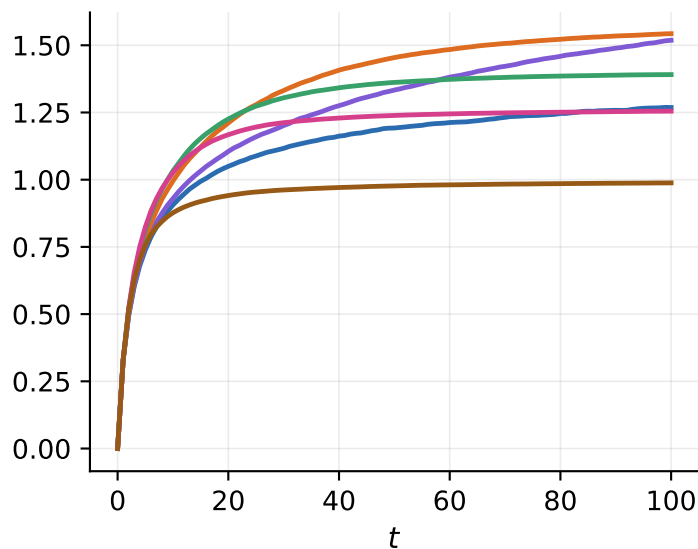
Uniform model U(-2, 2)
