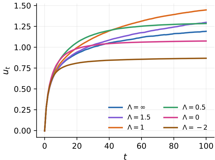
Gaussian model \mathcal{N}(0, 1)
