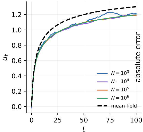
Gaussian model, \Lambda = \infty
