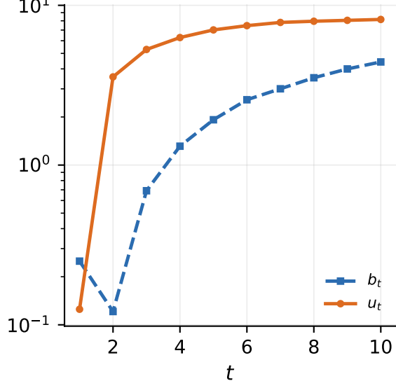
error at N = 10^6 , by step
