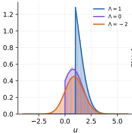
Gaussian model, t = 800
