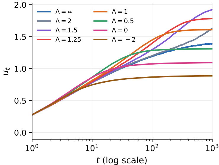
Gaussian \mathcal{N}(0, 1)
