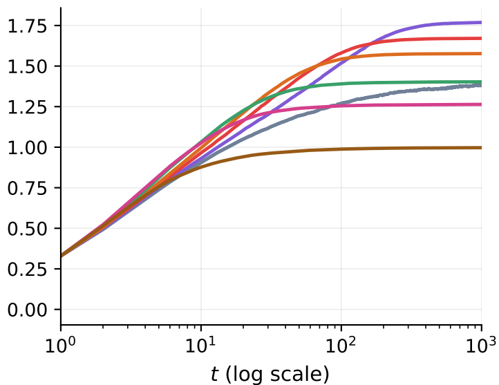
Uniform U(-2, 2)
