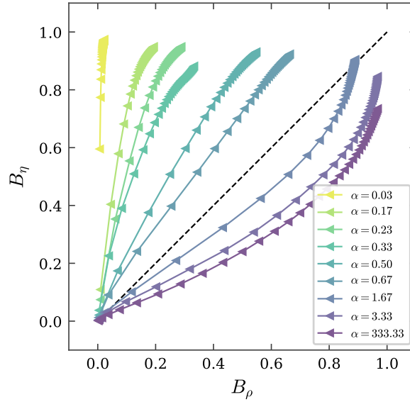
Figure 8: Which polarization comes first is set by the agenda. Trajectories in the (B_\rho, B_\eta) plane with no group bias ( b = 0 ), one curve per agenda complexity \alpha = P/K , markers equally spaced in time; they crowd at the end because the annealed dynamics slows, as §3.1 requires. Simple agendas run above the diagonal (distrust forms first), complex ones below it (disagreement first), crossing over at \alpha \approx 1.7 .
