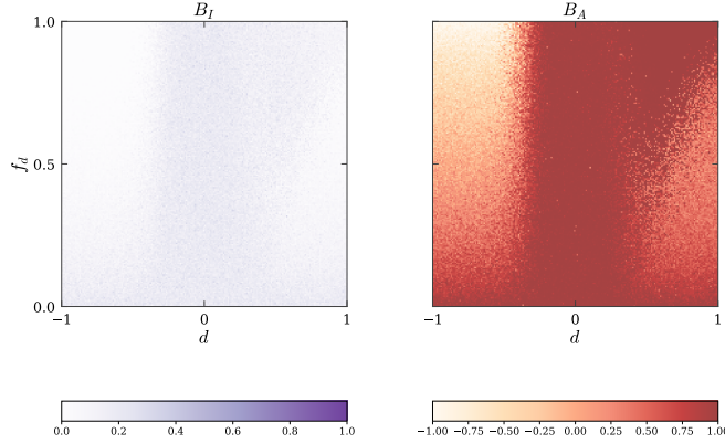
Figure 6: The two balance aggregates over the (d, f_d) plane , simple agenda ( \alpha = 0.17 ). B_A is the only measurement in the paper in which the frustrated region announces itself: at upper left it goes strongly negative, where every correlation merely goes to zero. B_I stays small everywhere, which is the conservation-law ceiling of Appendix A seen in this plane; for a complex agenda it saturates instead (Appendix B).
