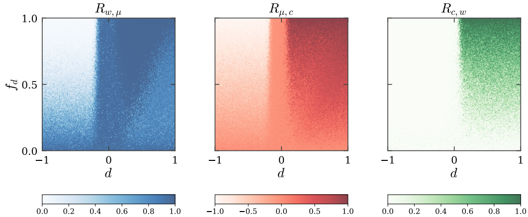
Figure 7: The three correlations , complex agenda ( \alpha = 3.3 ). Figure 4 for the other agenda size. R_{c,w} is the panel that changes: it now tracks R_{\mu,c} over most of the d > 0 half instead of remaining a fraction of it.
