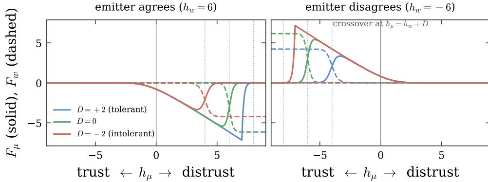
Figure 12: Cuts through the modulation functions at fixed opinion field, h_w = \pm 6 . Below the crossover at h_\mu = h_w + D the trust sector moves (solid, F_\mu ) and the receiver revises its trust; above it the opinion sector moves (dashed, F_w ) and the receiver unlearns what the emitter said. The discrimination field D displaces the crossover — dotted verticals, one per value of D — which is the entire mechanism studied in this paper, visible in a single coordinate.
