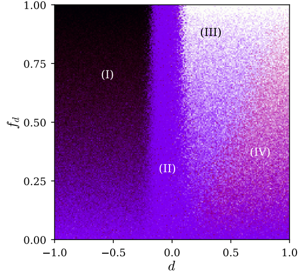
Figure 8: The phase diagram , complex agenda ( \alpha = 3.3 ): Figure 5 for the other agenda size. All four states are present. Region (III) now occupies the upper part of the discriminatory half, with (IV) confined to moderate f_d , where the discriminating fraction is still small enough that opinion has not caught up with trust.
