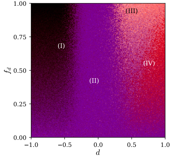
Figure 5: Four collective states. The three maps of Figure 4 combined as the red, green and blue channels of a single image — R_{\mu,c} the red, R_{c,w} the green, R_{w,\mu} the blue, each over the range its colour bar gives there. A colour therefore names a phase, and a dark pixel is one where all three correlations are small. (I) dark, frustrated favouring of the out-group: no correlation of any kind survives, which is why the balances of Figure 6 are needed to say what is there. (II) blue, opinion and trust correlated with each other but neither with class: neutral polarization. (III) pale, all three present, distrust and opinion both following the label. (IV) red, trust following the label without opinion: class alone. Simple agenda; the complex one has the same four states, with (III) taking a much larger share of the discriminatory half (Appendix B).
