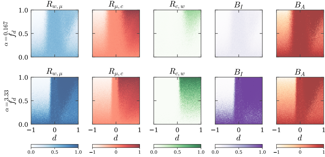
Figure 10: All five order parameters, both agendas , on one grid for reference: simple ( \alpha = 0.17 ) above, complex ( \alpha = 3.3 ) below.
