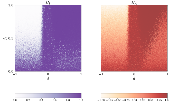
Figure 9: The two balance aggregates , complex agenda ( \alpha = 3.3 ): Figure 6 for the other agenda size. B_I saturates rather than staying near zero, which is what removes the ceiling on R_{c,w} . B_A is essentially unchanged, including the anti-balanced corner at upper left.
