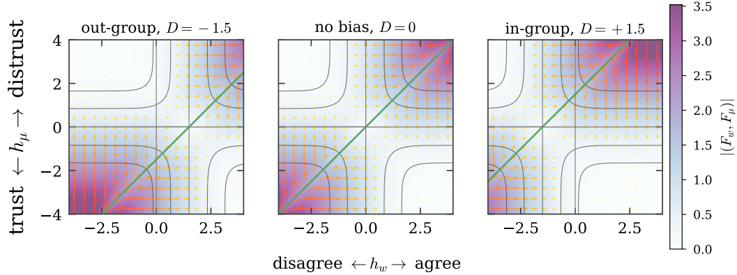
Figure 12: The discrimination field bends the flow of learning. Arrows are the change (F_w, F_\mu) that one interaction induces in the receiver’s fields; the background is |(F_w, F_\mu)| and the thin contours are the evidence Z . Centre: without discrimination the flow escapes the two dissonant quadrants into two symmetric consonant basins, separated by h_\mu = h_w (green). Left and right: a discriminating receiver evaluates the flow at h_w + D , which moves the separatrix and enlarges one basin at the other’s expense: “distrust and disagree” for an out-group emitter ( D = -d ), “trust and agree” for an in-group one ( D = +d ).
