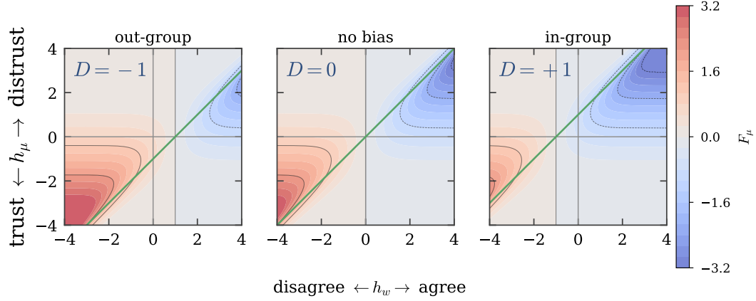
Figure 11: The discrimination field displaces the separatrix. F_\mu over the plane of Figure 1, for a receiver that sits at h_w but evaluates the modulation at h_w + D : the axes stay put and the green separatrix h_\mu = h_w + D slides. Centre, no bias, and the two halves are balanced. Left, an out-group emitter under d > 0 : the red region, where F_\mu > 0 and distrust grows, takes more of the plane. Right, an in-group emitter: the blue region, where trust grows, takes it instead. F_\mu is the function to watch because the field enters through h_w , and it is the prefactor 1 - 2\Phi(h_w) in F_\mu that carries it into the trust sector.
