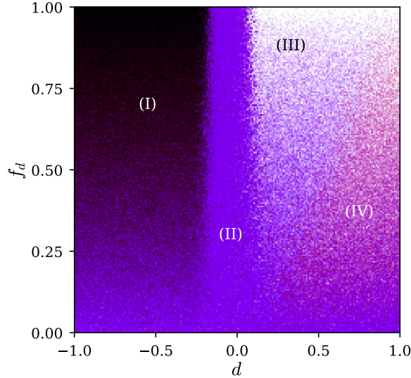
Figure 7: The phase diagram , complex agenda ( \alpha = 3.3 ): Figure 5 for the other agenda size. All four states are present. Region (III) now occupies the upper part of the discriminatory half, with (IV) confined to moderate f_d , where the discriminating fraction is still small enough that opinion has not caught up with trust.
