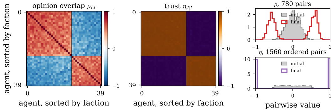
Figure 2: An unbiased society splits into two mutually distrustful camps. One society of N = 40 agents at d = 0 , simple agenda. Left and centre: the opinion overlap \rho_{IJ} and the trust \eta_{JI} at the end of the run, every agent against every other, with agents ordered by the leading eigenvector of \rho and the line marking where the two factions meet — here 24 agents against 16, a split with no label behind it. Agreement and trust inside the blocks, disagreement and distrust across them. Right: the distributions over all pairs, which need no ordering and so cannot be an artefact of it. Opinion overlap (780 unordered pairs) starts unimodal at zero, the width 1/\sqrt{K} of random vectors in K = 30 dimensions, and ends bimodal near \pm 0.6 . Trust (1560 ordered pairs) starts spread over the interior and ends saturated at \pm 1 : the two-tone matrix in the centre is made by the dynamics, not by the initial condition. The two sectors are shown on separate axes because they saturate to very different degrees, for the reason given in §4.
