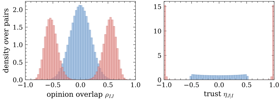
Figure 2: An unbiased society splits in two. Eight independent societies of N = 400 agents at d = 0 , simple agenda, before and after the calibrated 500 interactions per ordered pair, with their pairs pooled: 638 400 unordered pairs for the opinion overlap and 1 276 800 ordered pairs for the trust. Blue is the initial state, red the final one. Neither panel depends on how the agents are labelled, so neither can be an artefact of sorting them. Opinion overlap starts unimodal at zero, of width 1/\sqrt{K} as random vectors in K = 30 dimensions require, and ends bimodal; trust starts spread across the interior and ends saturated at \pm 1 , so the split in trust is built by the dynamics and not supplied by the initial condition. Bimodality alone would show only that every pair has taken a side; that the sides are exactly two blocs is the sign-balance figure quoted in the text.
