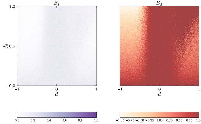
Figure 8: The two balance aggregates , simple agenda ( \alpha = 0.17 ). B_A is the only measurement in the paper in which the frustrated region announces itself, going strongly negative at upper left where every correlation merely goes to zero. B_I stays small everywhere.
