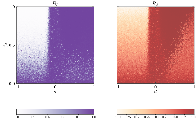
Figure 9: The two balance aggregates , complex agenda ( \alpha = 3.3 ). B_I saturates rather than staying near zero, which is what removes the ceiling on R_{c,w} . B_A is essentially unchanged, including the anti-balanced corner at upper left.
