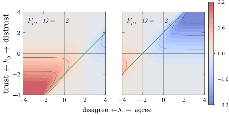
Figure 11: The discrimination field displaces the separatrix. F_\mu over the same plane and in the same layout as Figure 1, for a discriminating receiver: it sits at h_w but evaluates the modulation at h_w + D , so the green separatrix h_\mu = h_w + D slides while the axes stay put. F_\mu is the function to watch, because the field enters through h_w and it is the prefactor 1 - 2\Phi(h_w) in F_\mu that carries it into the trust sector. Left, an out-group emitter under d > 0 : the red region, where distrust grows, takes most of the plane. Right, an in-group emitter: the blue region, where trust grows, takes it instead. Compare Figure 1, where the line runs through the origin and the two are balanced. This is the whole mechanism of the paper: every discriminating agent is biased towards the same alignment of distrust with class, and the flow that results is Figure 12.
